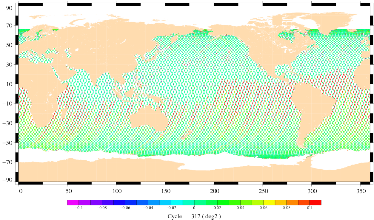
Square of the off nadir angle from waveforms Jason-1 Cycle 317 (09/08/2010 / 19/08/2010)
