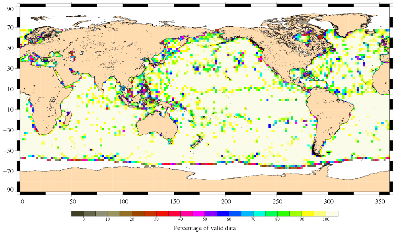
Percentage of valid data relative to the nominal pass Jason-1 Cycle 317 (09/08/2010 / 19/08/2010)
