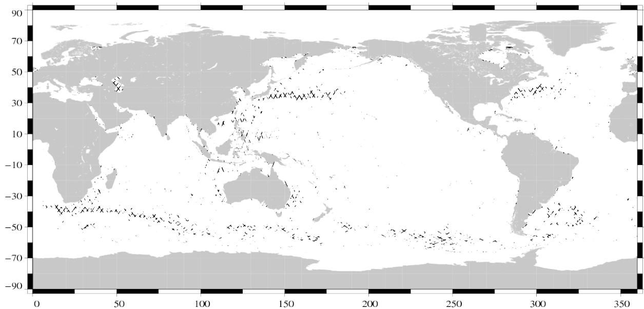
Valid data: (SSH – MSS) differences greater than 30 cm Jason-1 Cycle 317 (09/08/2010 / 19/08/2010)
