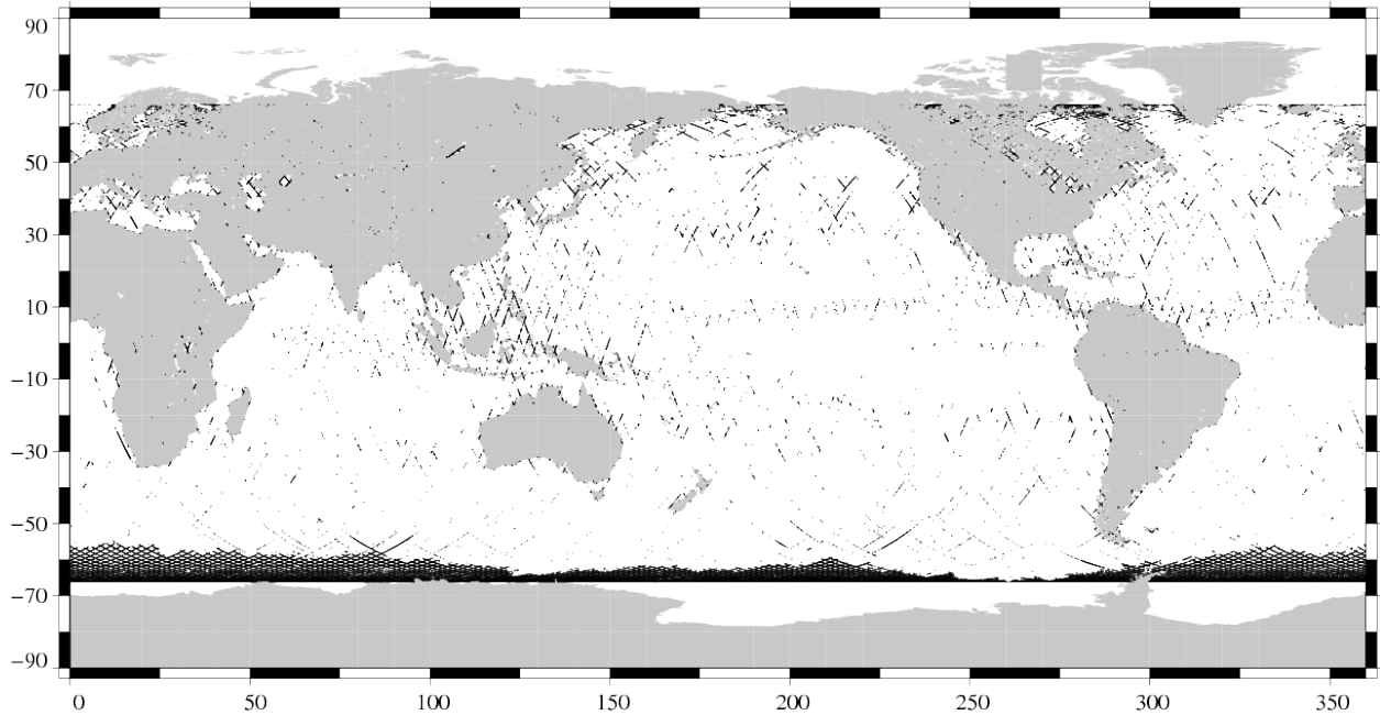
Valid data Jason-1 Cycle 317 (09/08/2010 / 19/08/2010)
