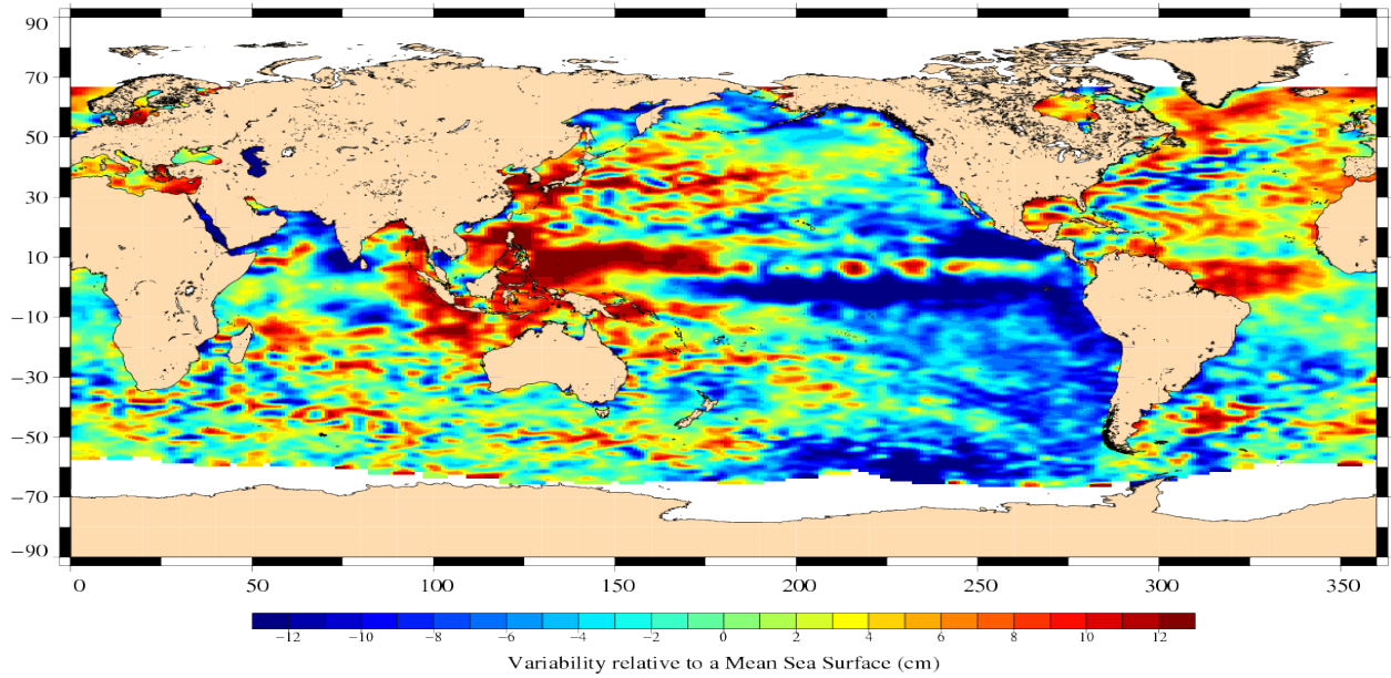
Jason-1 Cycle 319 29/08/2010 – 08/09/2010
