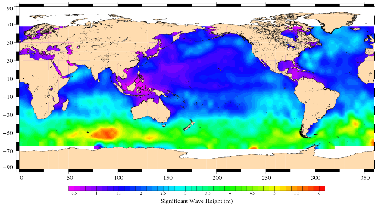
Jason-1 Cycle 319 29/08/2010 – 08/09/2010
