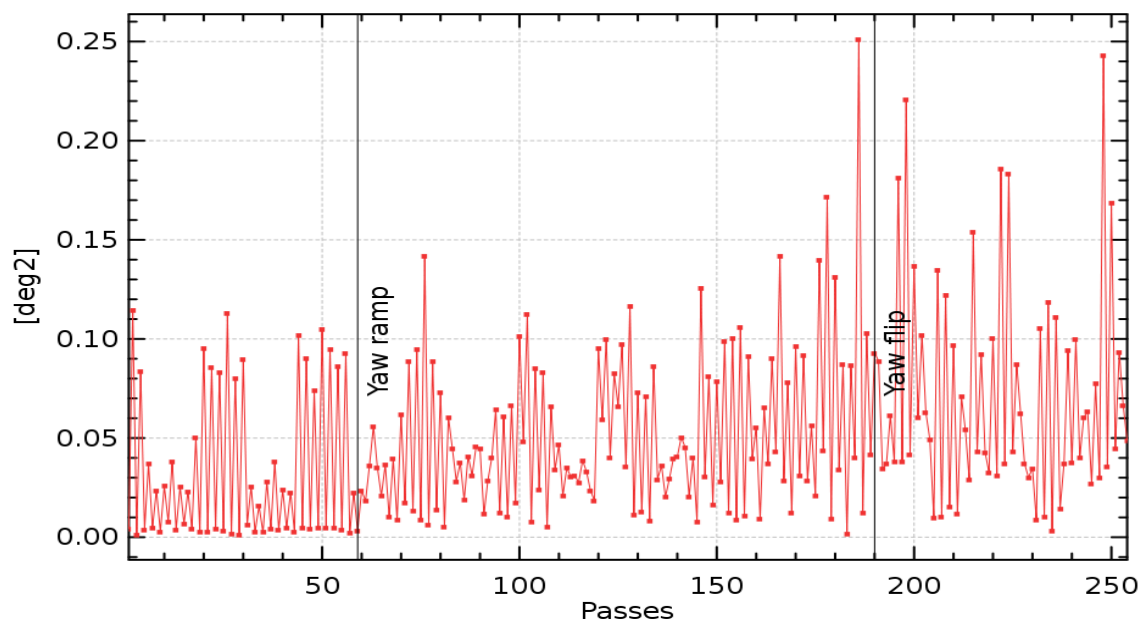
GDR Jason-1 Cycle 321: Mean by pass of apparent squared mispointing
