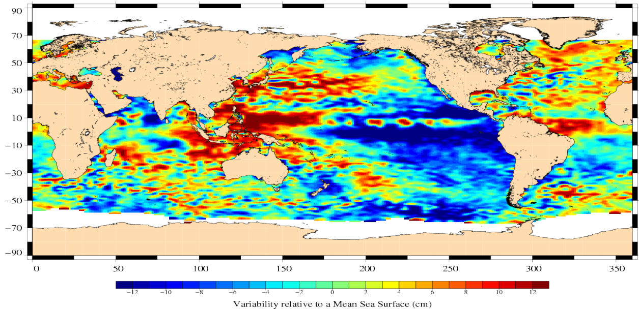
Jason-1 Cycle 321 18/09/2010 – 28/09/2010
