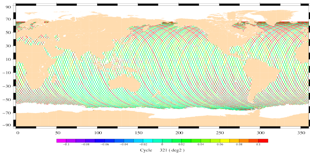
GDR Jason-1 Cycle 321: Mean by pass of apparent squared mispointing
