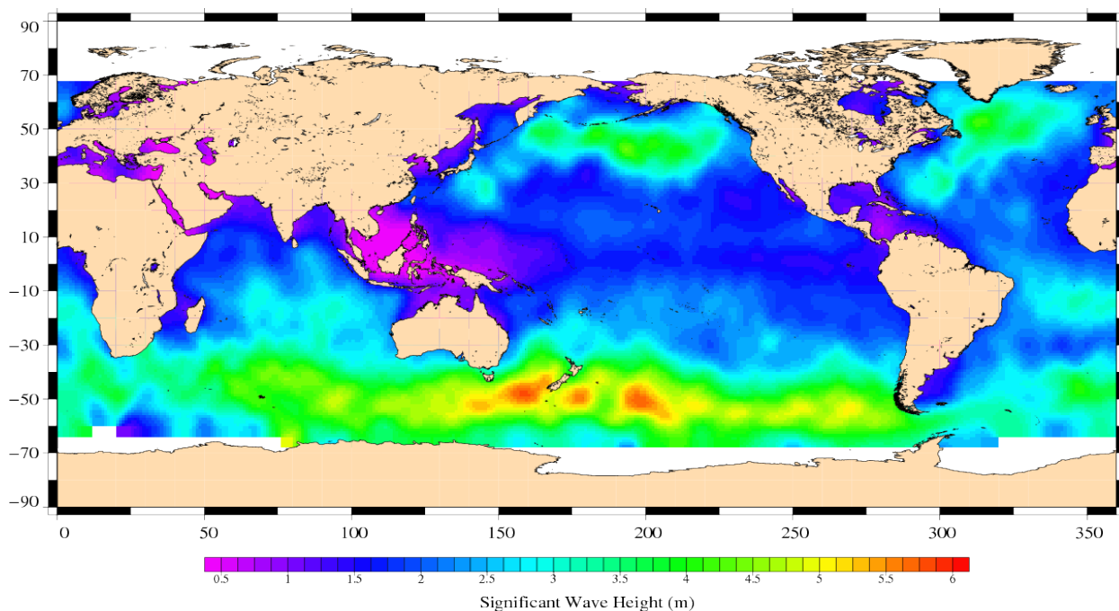
Jason-1 Cycle 321 18/09/2010 – 28/09/2010
