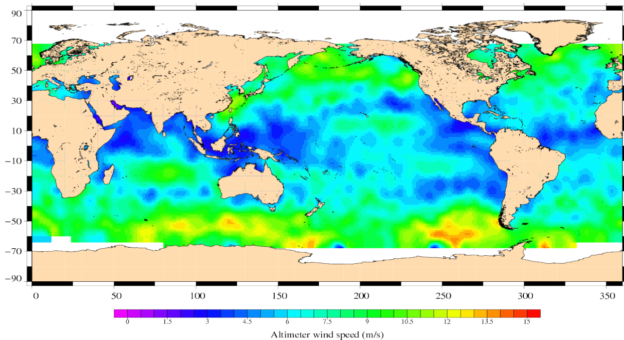
Jason-1 Cycle 324 18/10/2010 – 27/10/2010
