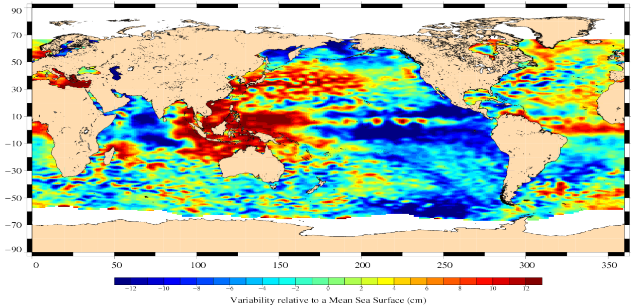
Jason-1 Cycle 324 18/10/2010 – 27/10/2010
