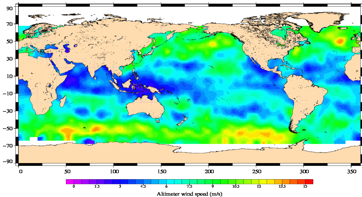
Jason-1 Cycle 326 06/11/2010 - 16/11/2010
