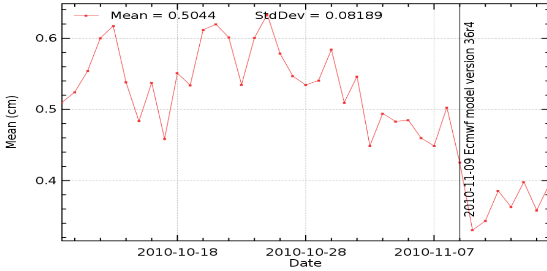
Gdr Jason-1: Daily mean of radiometer - ECMWF model wet troposphere correction
