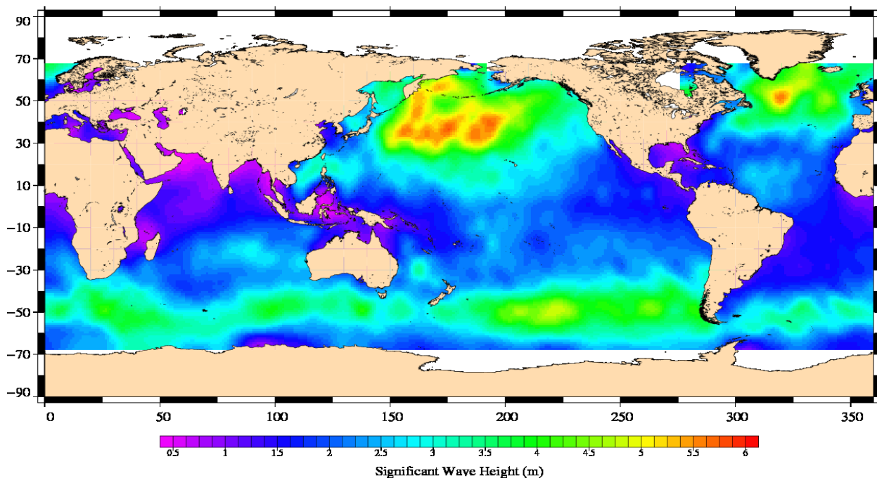
Jason-1 Cycle 333 15/01/2011 – 25/01/2011
