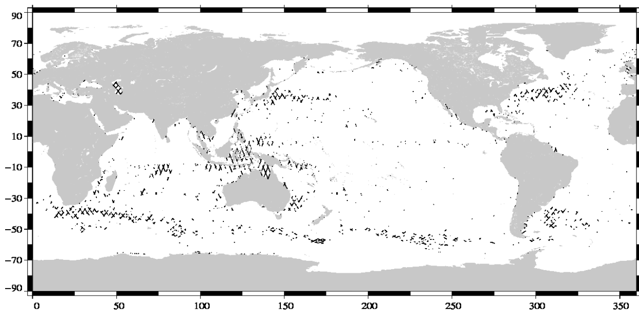
Valid data: (SSH – MSS) differences greater than 30 cm Jason-1 Cycle 338 (05/03/2011 / 15/03/2011)
