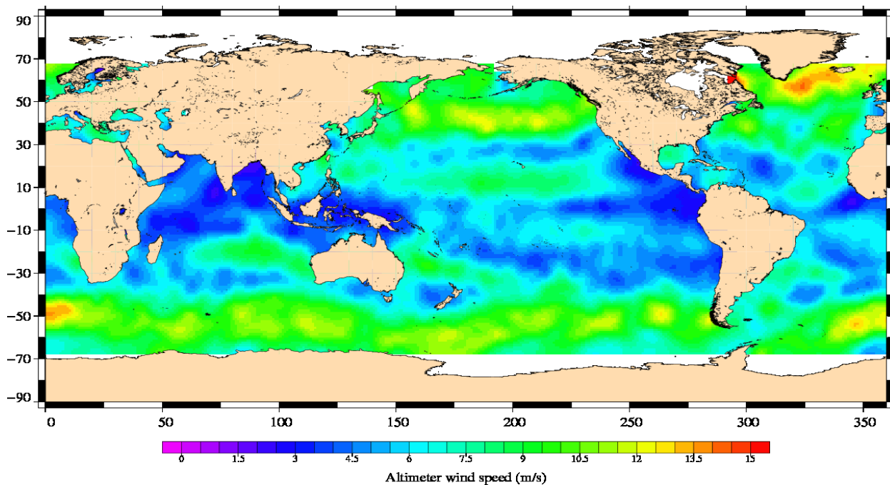
Jason-1 Cycle 338 05/03/2011 – 15/03/2011
