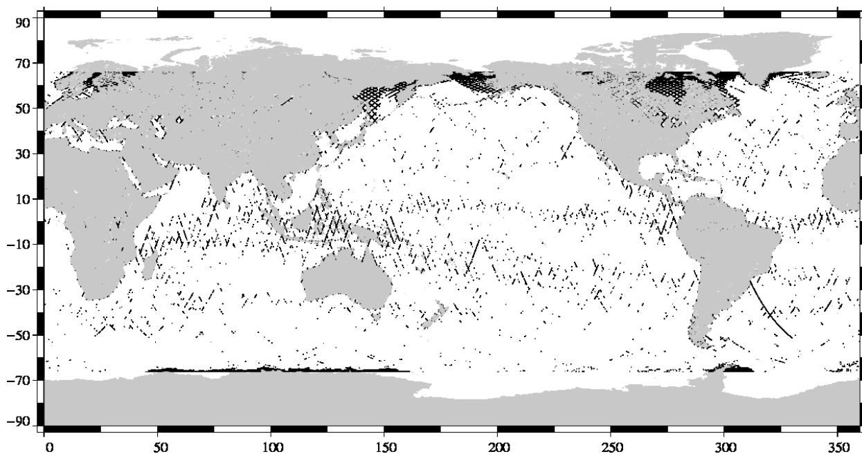
Edited measurements Jason-1 Cycle 338 (05/03/2011 / 15/03/2011)
