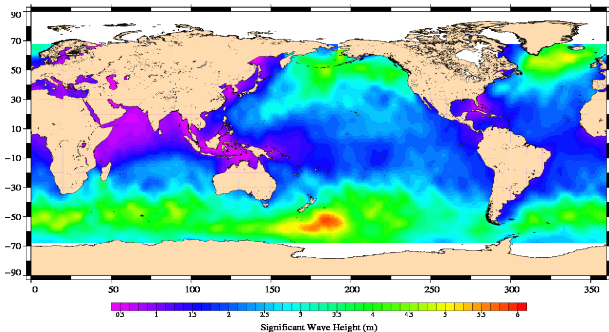
Jason-1 Cycle 341 04/04/2011 - 14/04/2011
