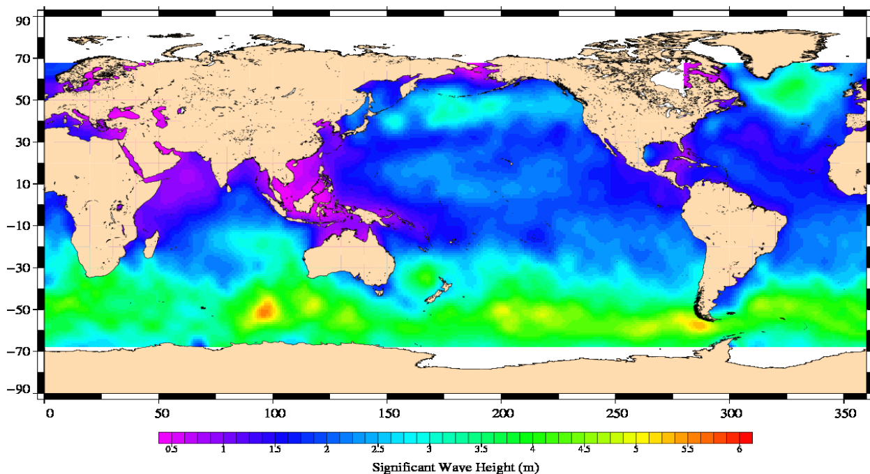
Jason-1 Cycle 343 24/04/2011 - 04/05/2011
