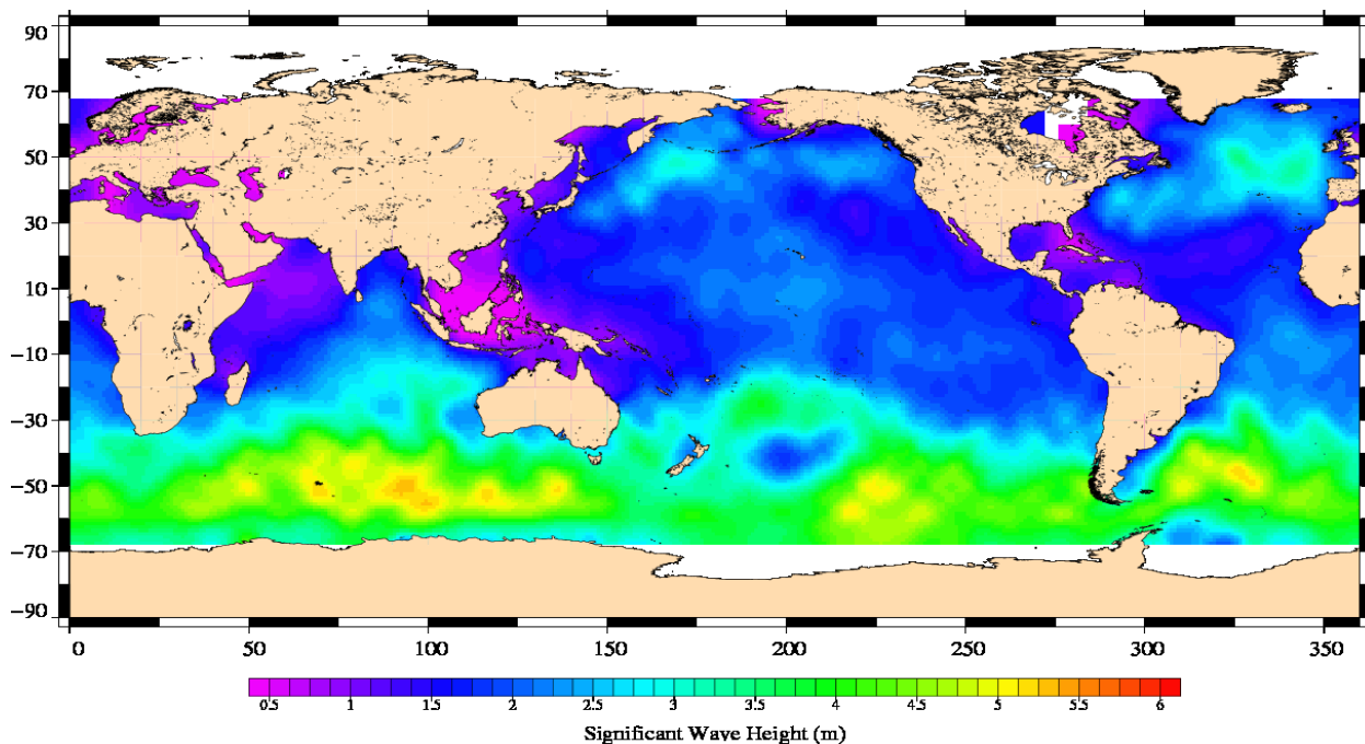
Jason-1 Cycle 344 04/05/2011 - 14/05/2011
