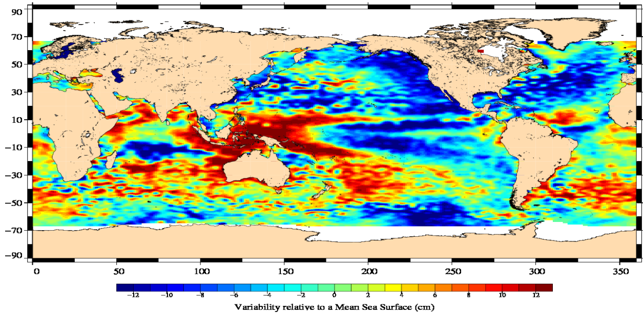
Jason-1 Cycle 344 04/05/2011 – 14/05/2011
