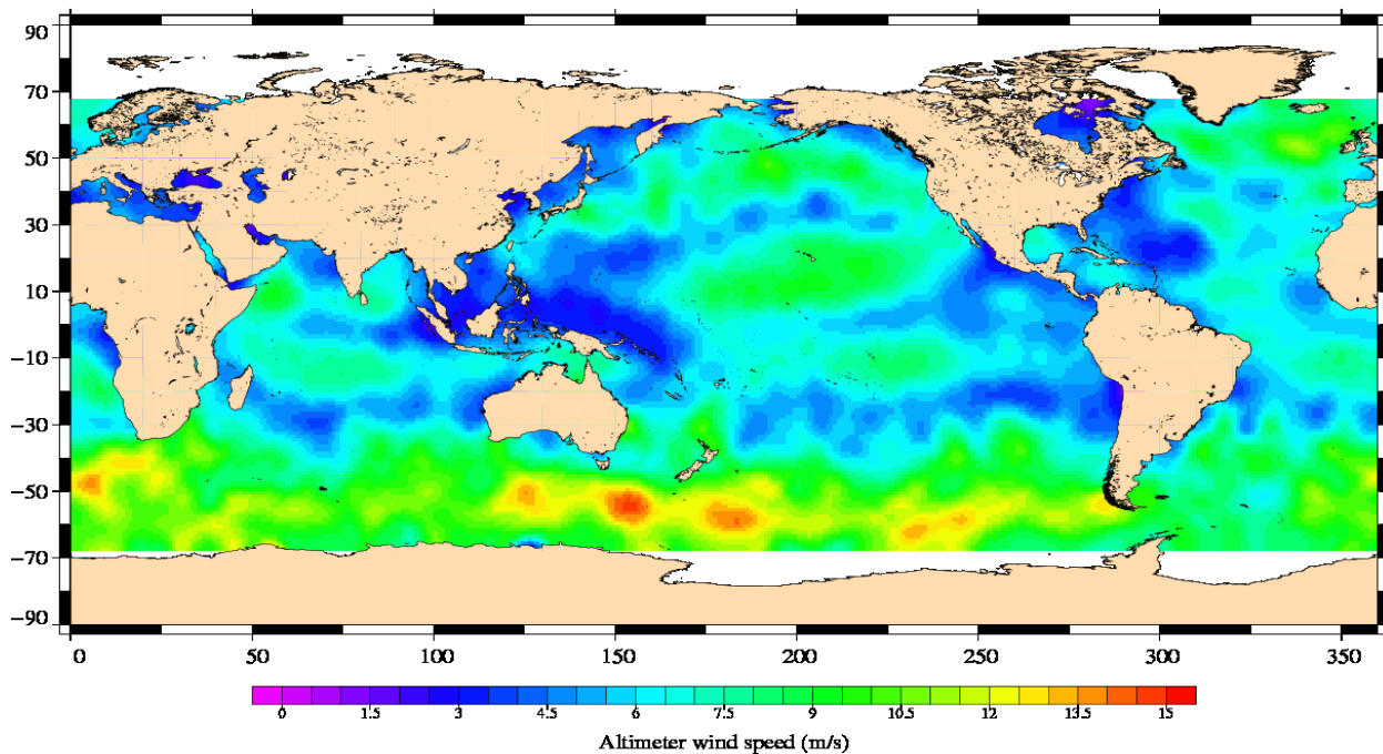
Jason-1 Cycle 346 24/05/2011 – 03/06/2011
