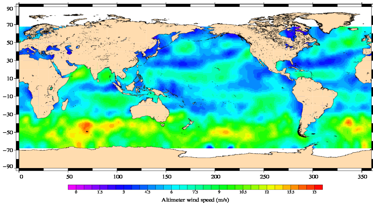
Jason-1 Cycle 348 12/06/2011 – 22/06/2011
