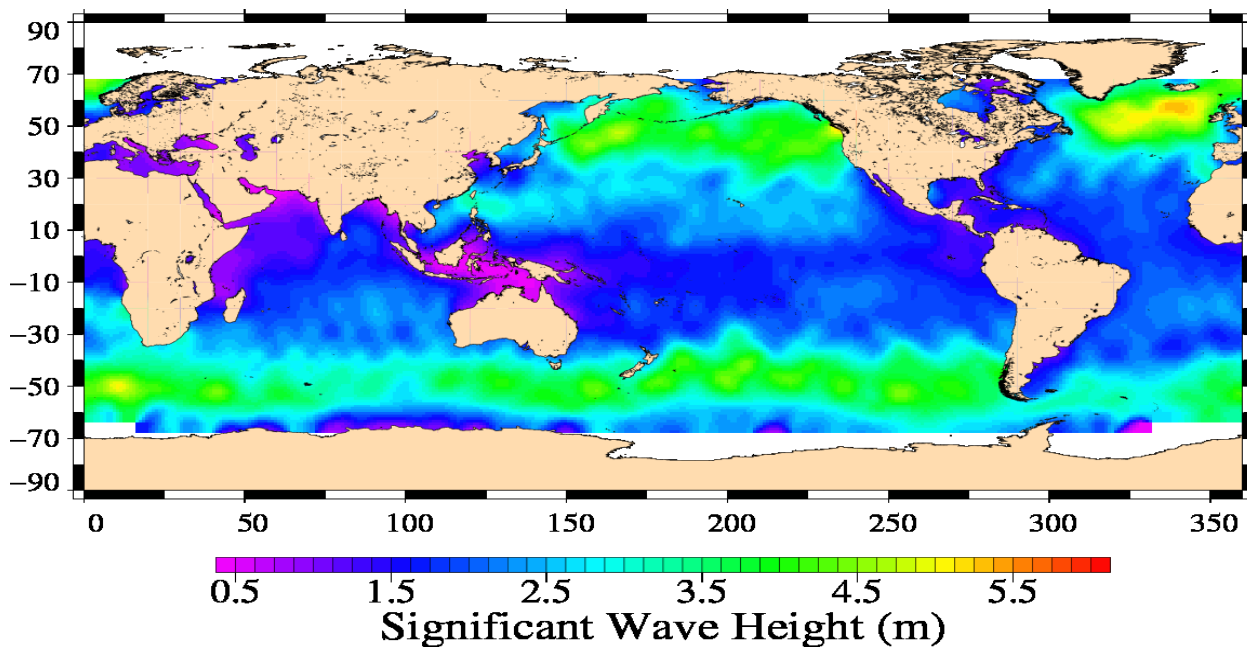
Jason-1 Cycle 364 18/11/2011 – 28/11/2011
