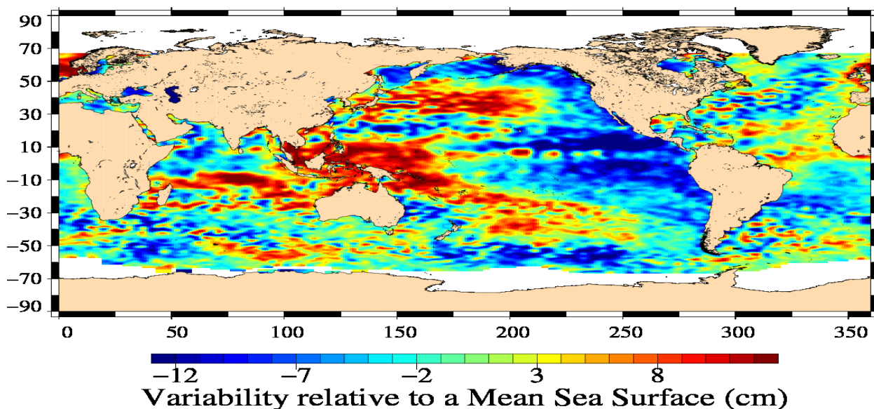
Jason-1 Cycle 364 18/11/2011 – 28/11/2011
