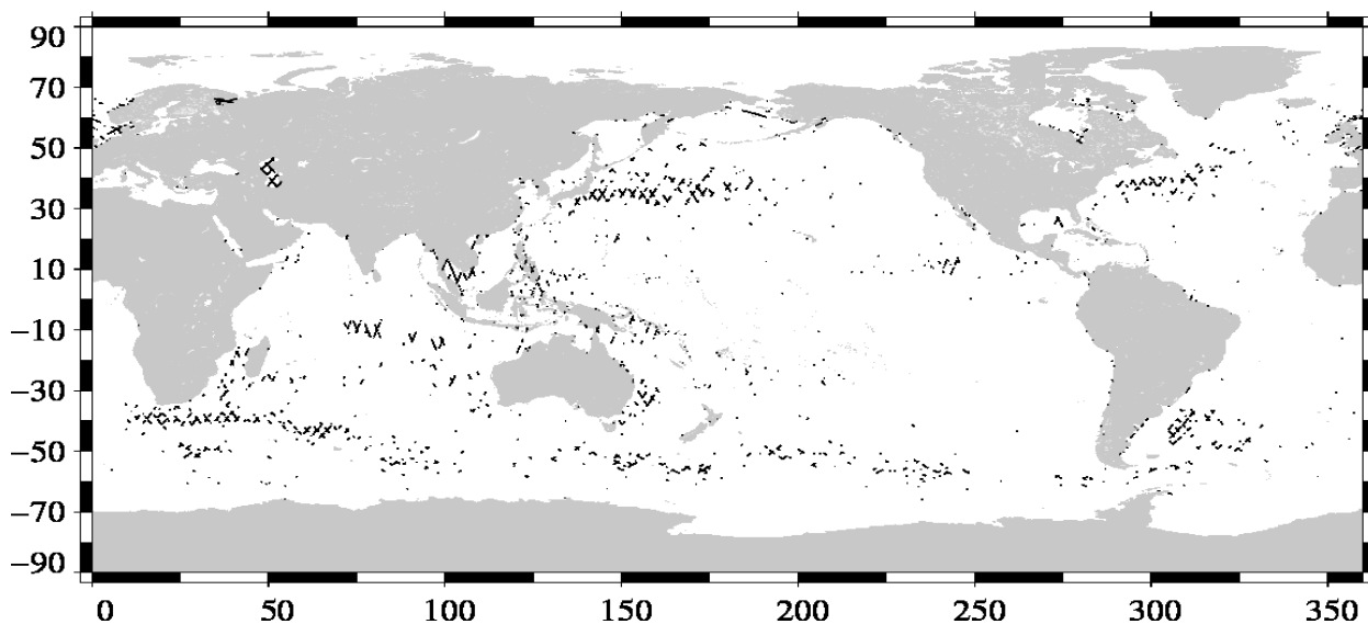
Valid data: (SSH – MSS) differences greater than 30 cm Jason-1 Cycle 364 (18/11/2011 / 28/11/2011)
