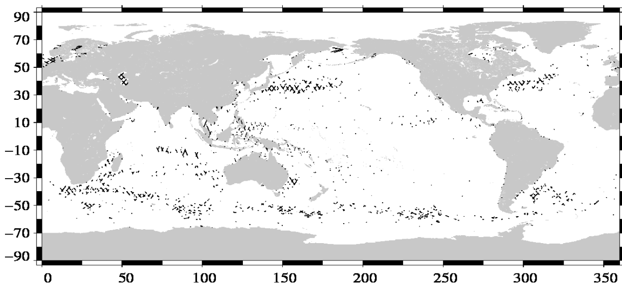
Valid data: (SSH – MSS) differences greater than 30 cm Jason-1 Cycle 365 (28/11/2011 / 08/12/2011)
