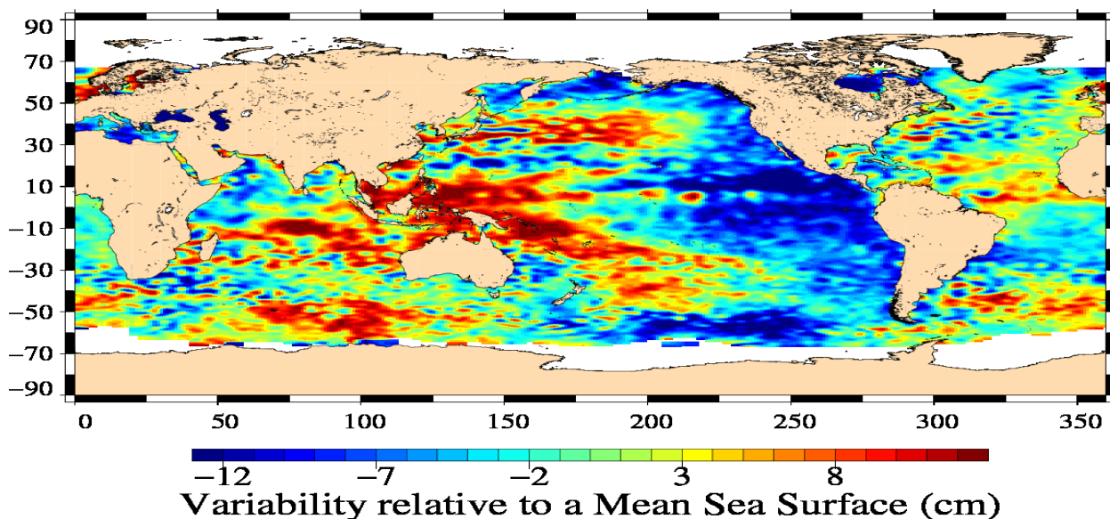
Jason-1 Cycle 365 28/11/2011 – 08/12/2011
