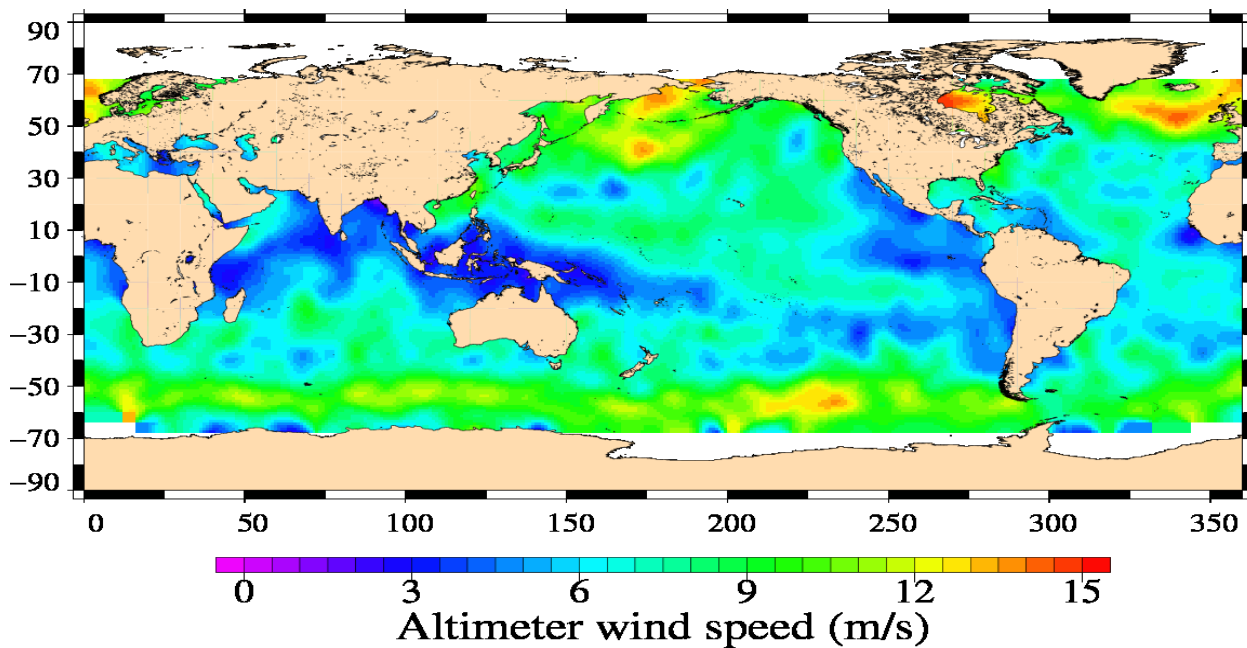
Jason-1 Cycle 365 28/11/2011 – 08/12/2011
