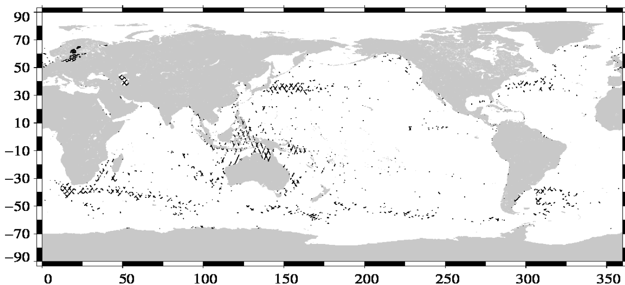
Valid data: (SSH – MSS) differences greater than 30 cm Jason-1 Cycle 370 (17/01/2012 / 27/01/2012)
