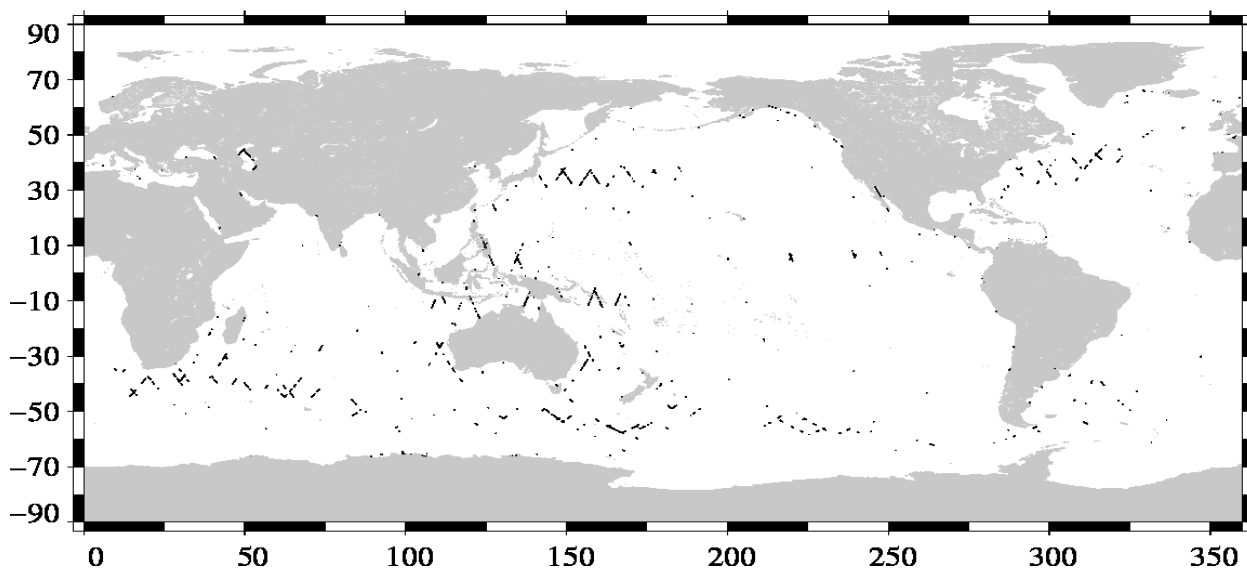
Valid data: (SSH – MSS) differences greater than 30 cm Jason-1 Cycle 374 (29/02/2012 / 03/03/2012)
