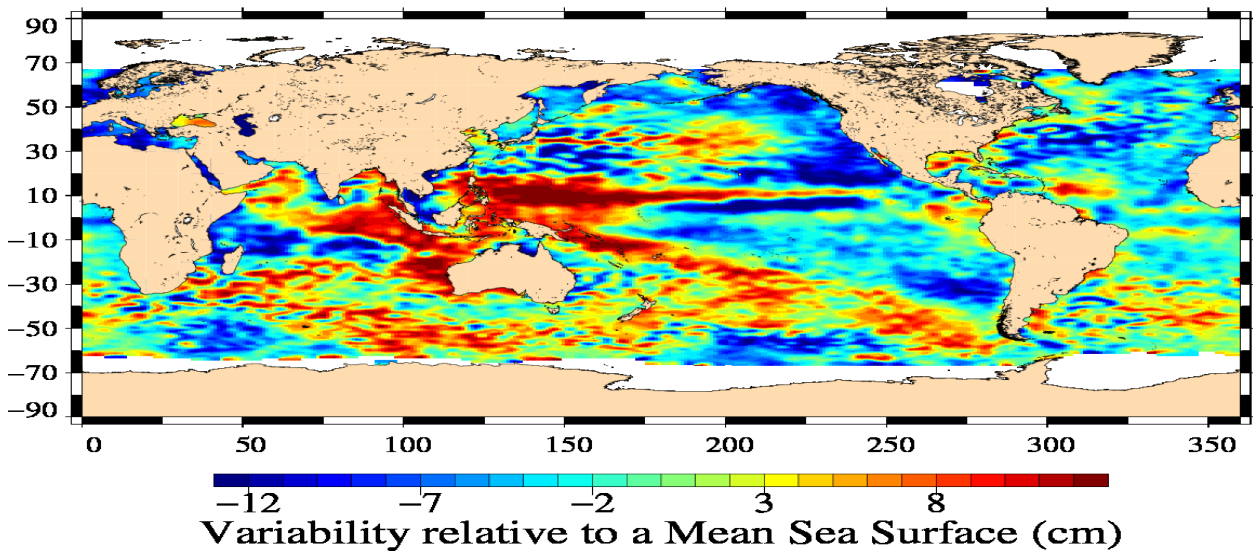
Jason-1 Cycle 503 09/06/2012 – 20/06/2012
