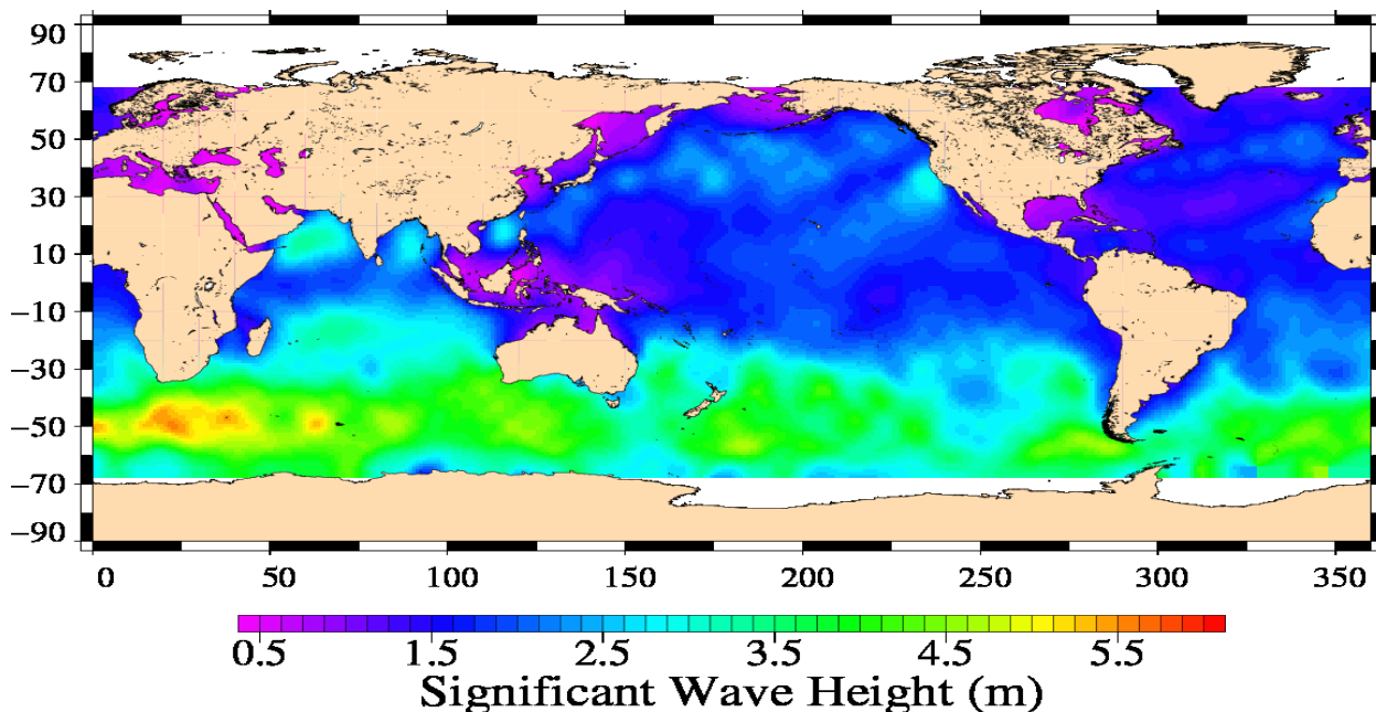
Jason-1 Cycle 503 09/06/2012 – 20/06/2012
