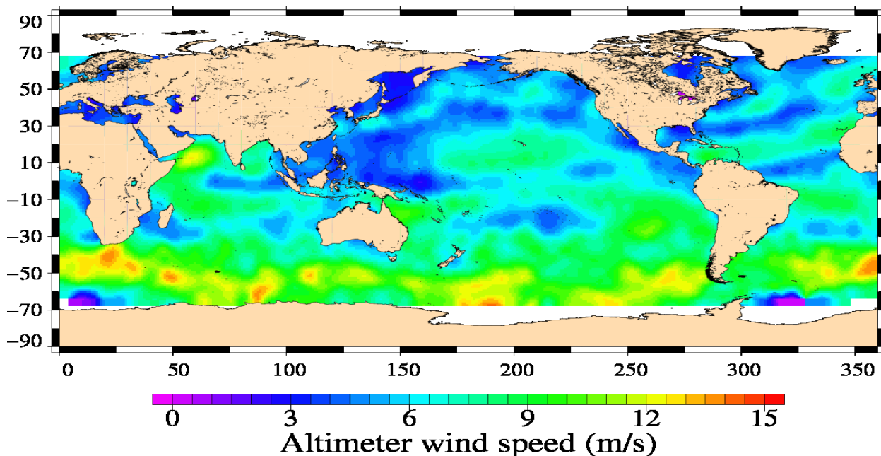
Jason-1 Cycle 505 01/07/2012 – 12/07/2012
