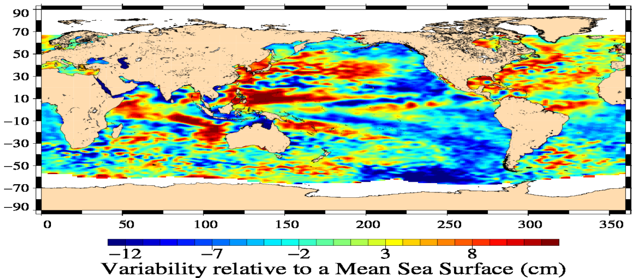
Jason-1 Cycle 509 13/08/2012 – 24/08/2012
