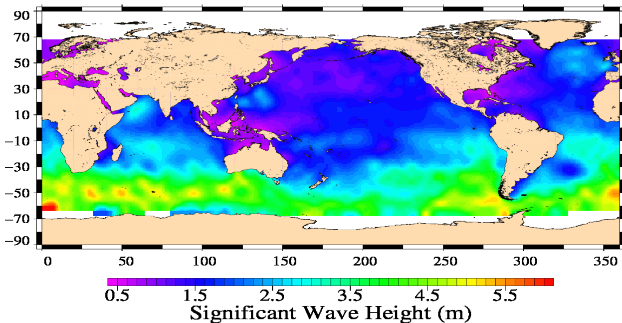
Jason-1 Cycle 509 13/08/2012 – 24/08/2012
