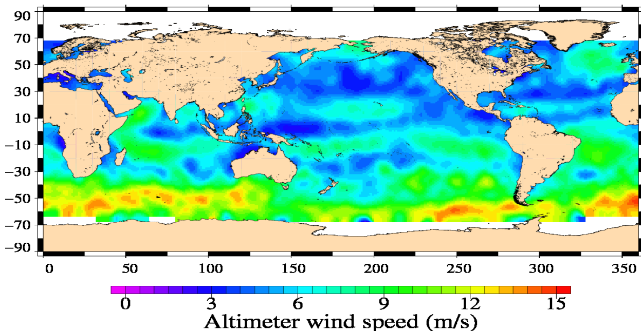
Jason-1 Cycle 509 13/08/2012 – 24/08/2012
