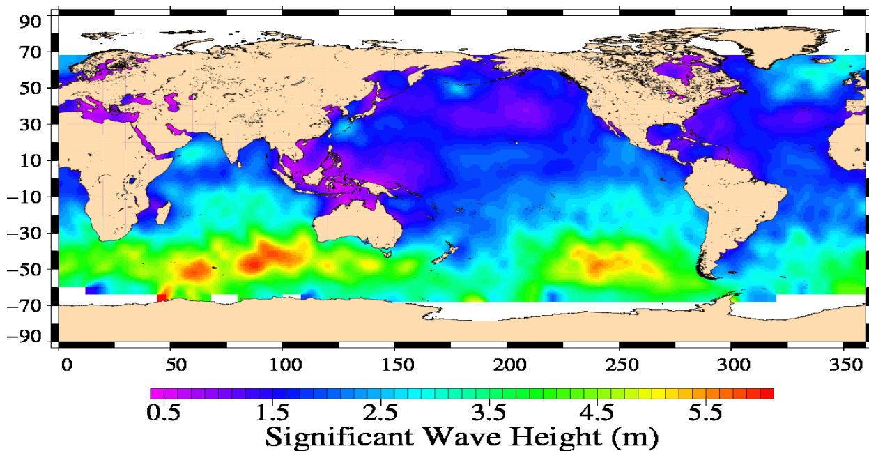
Jason-1 Cycle 510 24/08/2012 – 04/09/2012
