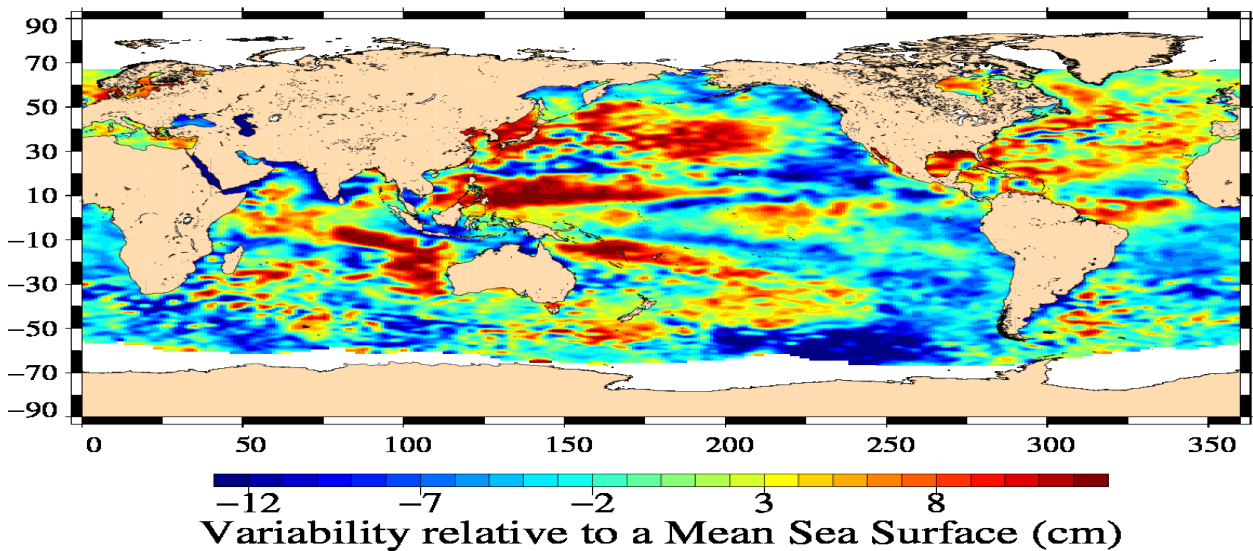
Jason-1 Cycle 510 24/08/2012 – 04/09/2012
