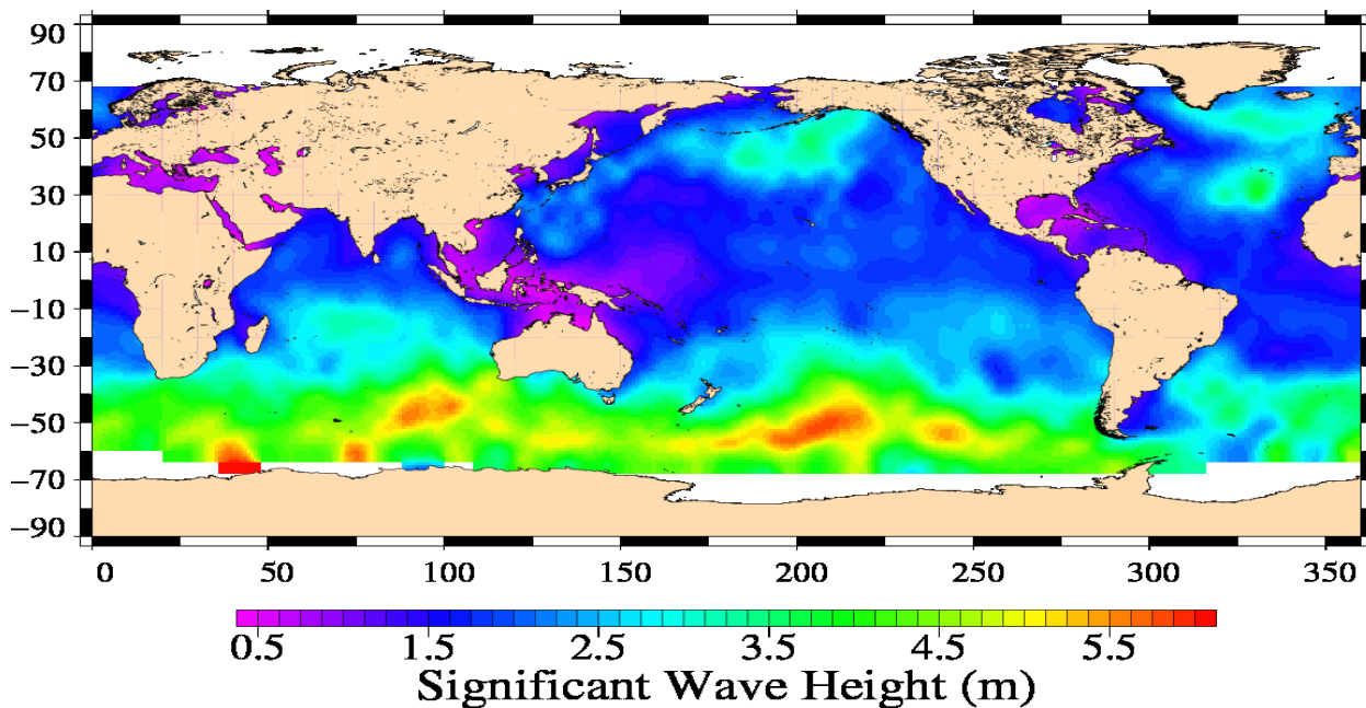
Jason-1 Cycle 512 15/09/2012 – 26/09/2012
