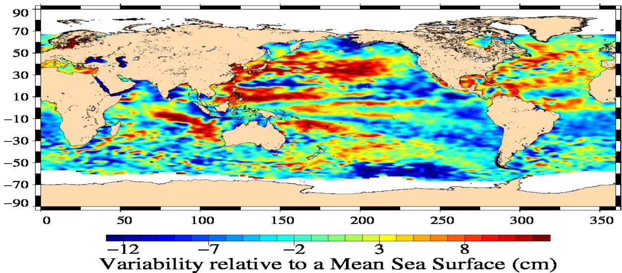
Jason-1 Cycle 512 15/09/2012 – 26/09/2012
