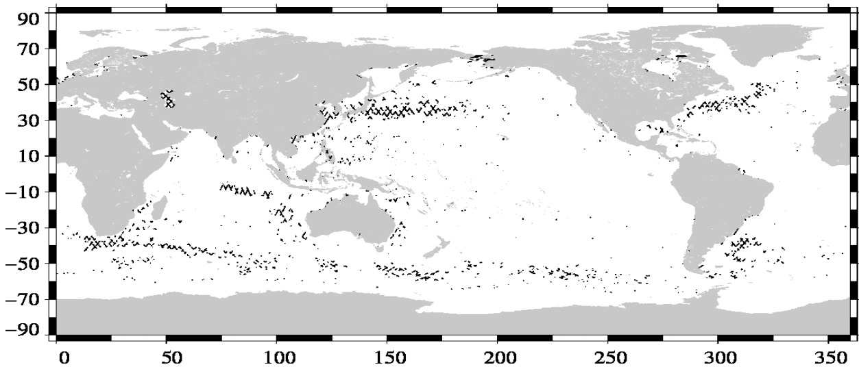
Valid data: (SSH – MSS) differences greater than 30 cm Jason-1 Cycle 513 (26/09/2012 / 07/10/2012)
