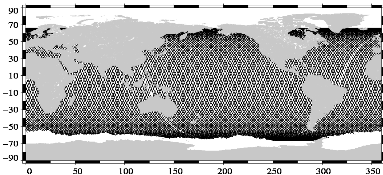
Valid data Jason-1 Cycle 513 (26/09/2012 / 07/10/2012)
