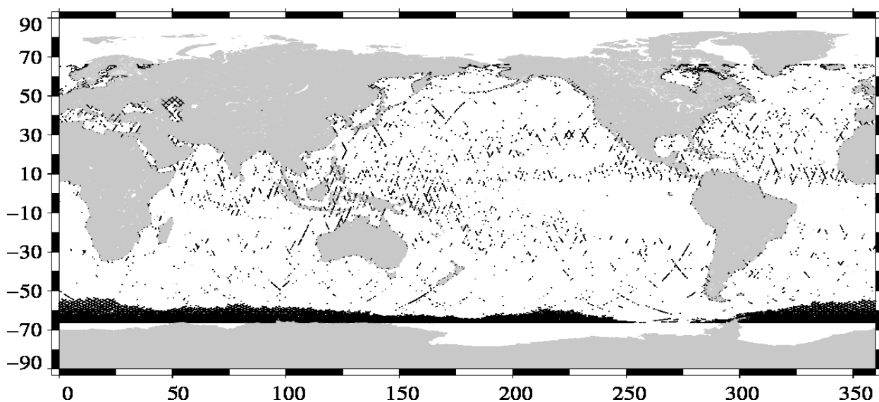
Edited measurements Jason-1 Cycle 513 (26/09/2012 / 07/10/2012)
