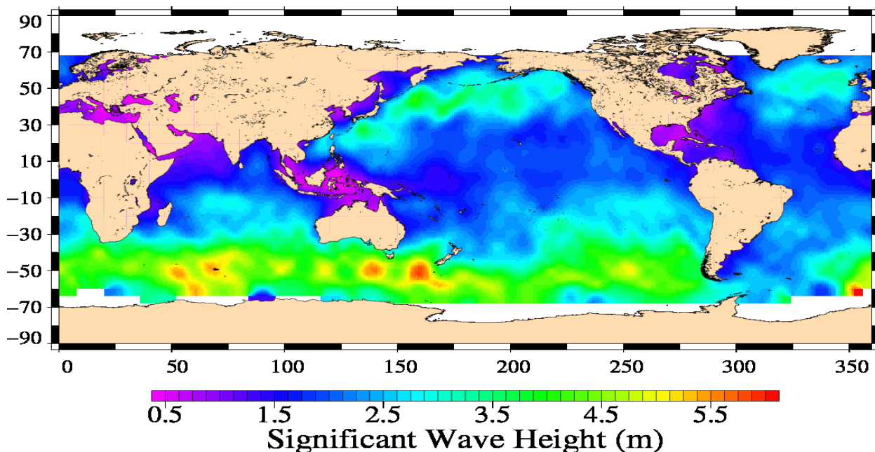
Jason-1 Cycle 513 26/09/2012 – 07/10/2012
