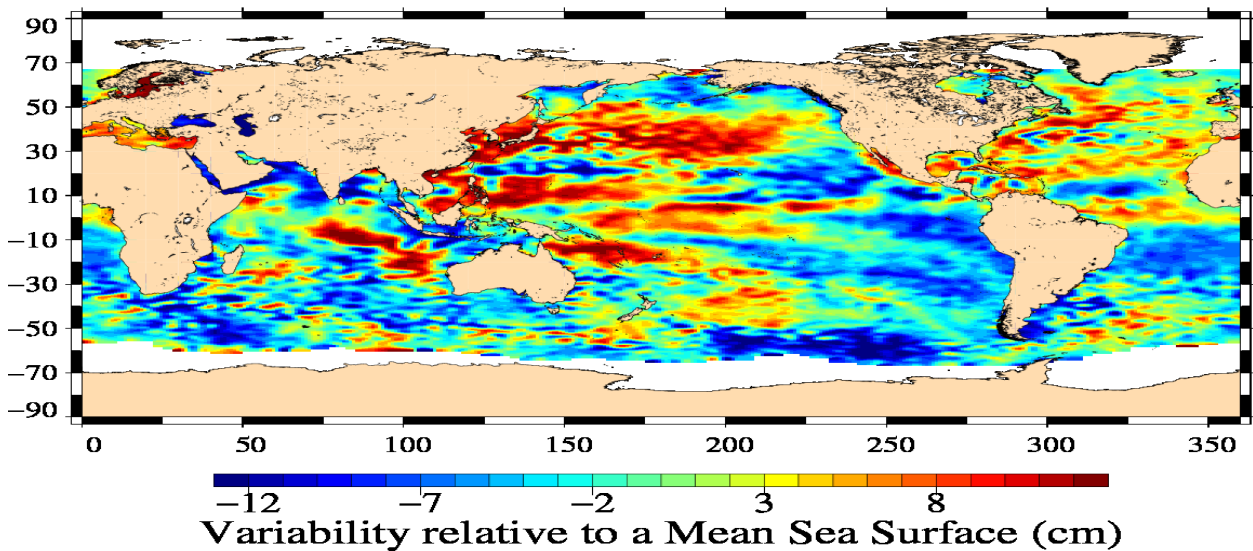
Jason-1 Cycle 513 26/09/2012 – 07/10/2012
