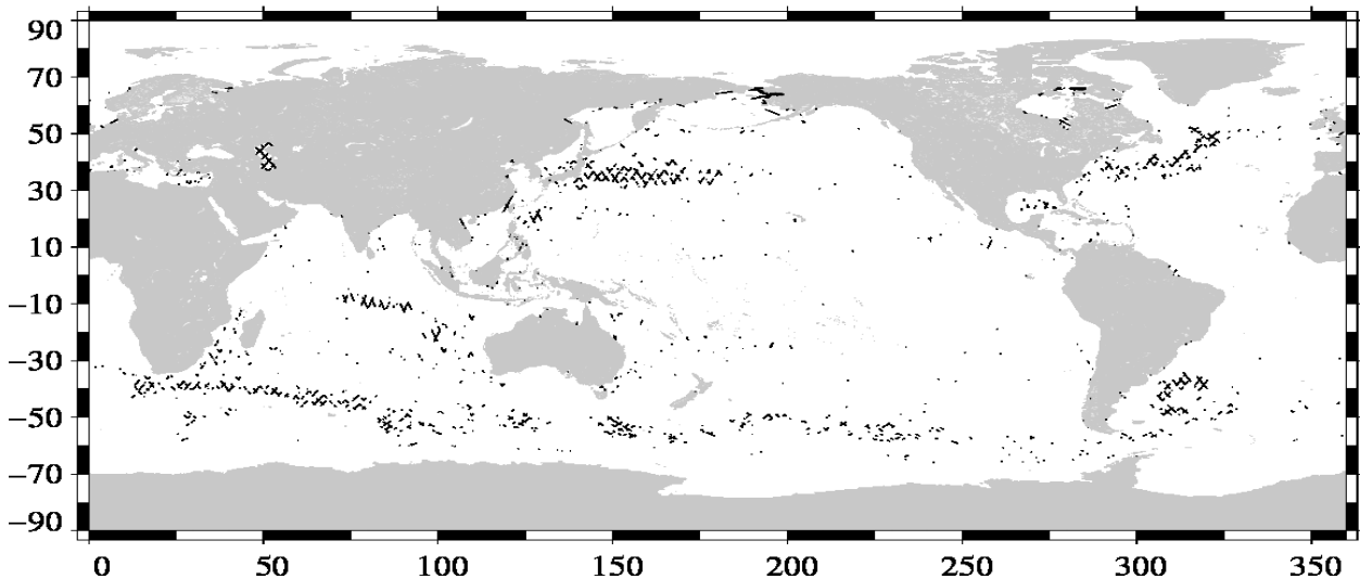
Valid data: (SSH – MSS) differences greater than 30 cm Jason-1 Cycle 516 (29/10/2012 / 08/11/2012)
