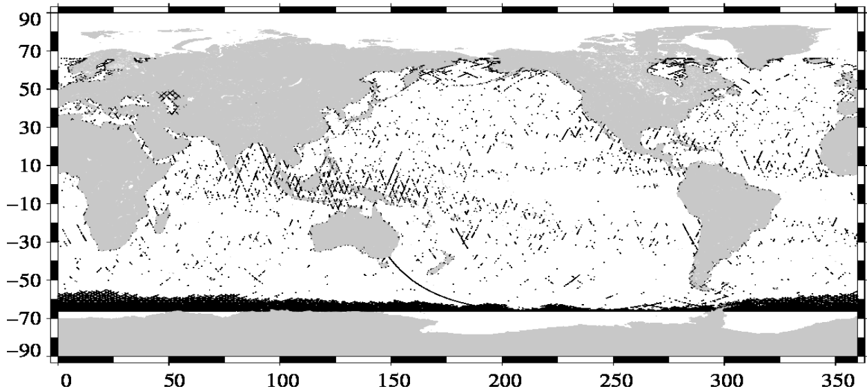
Edited measurements Jason-1 Cycle 516 (29/10/2012 / 08/11/2012)
