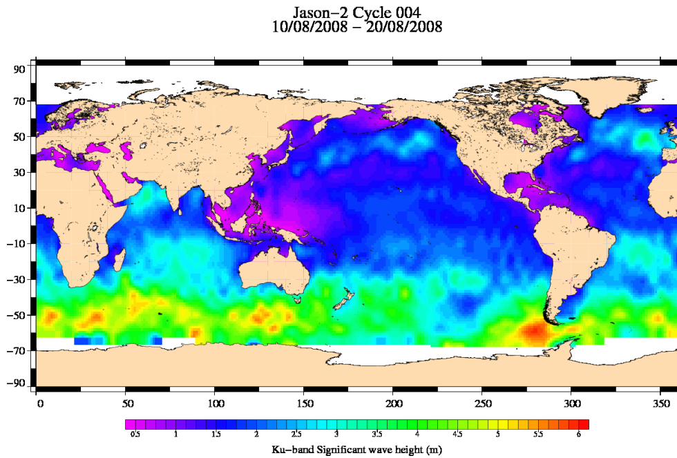
FIG. 5 – Significant wave height for cycle 004.
