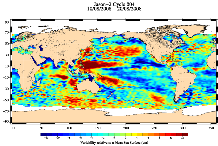
FIG. 18 – Sea level anomaly relative to MSS for cycle 004.
