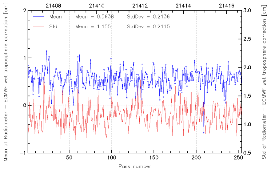
FIG. 11 – Pass monitoring of wet troposphere differences between radiometer and ECMWF model for Jason-2 cycle 004.
