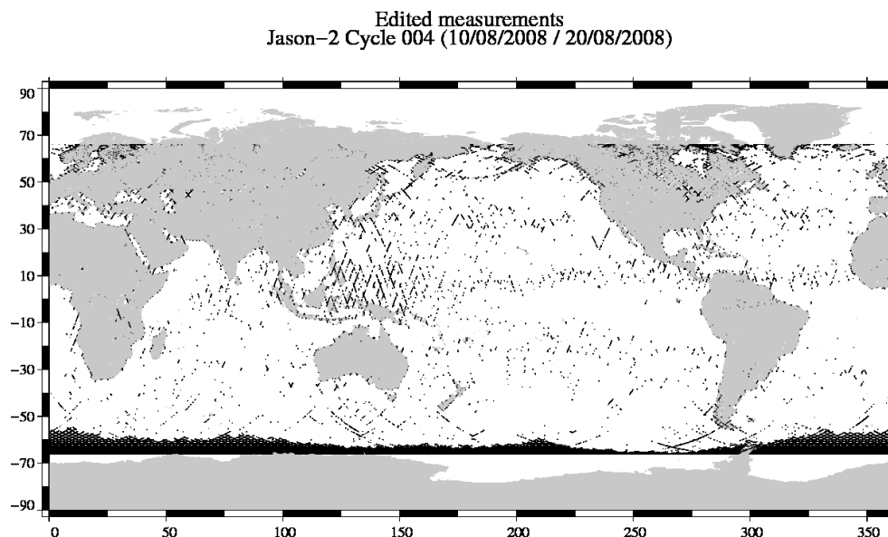
FIG. 2 – Edited measurements for cycle 004.
