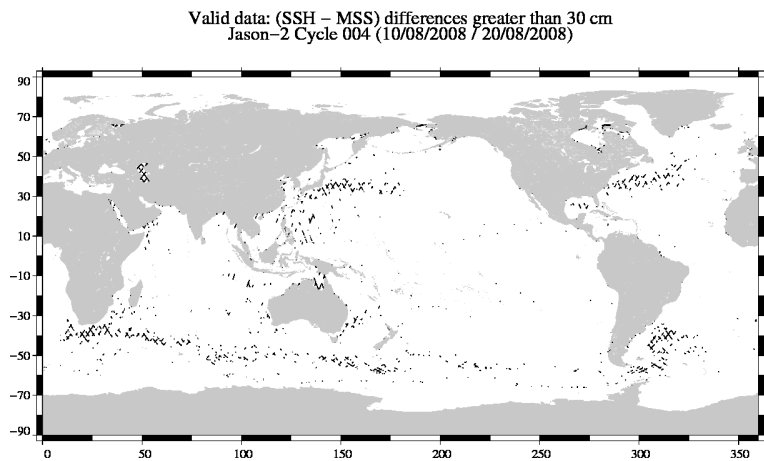
FIG. 19 – Differences higher than a 30 cm threshold for cycle 004.
