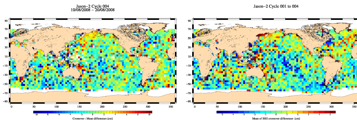
FIG. 13 – Mean SSH at crossovers for cycle 004 (left) and over the whole Jason-2 period (right).
