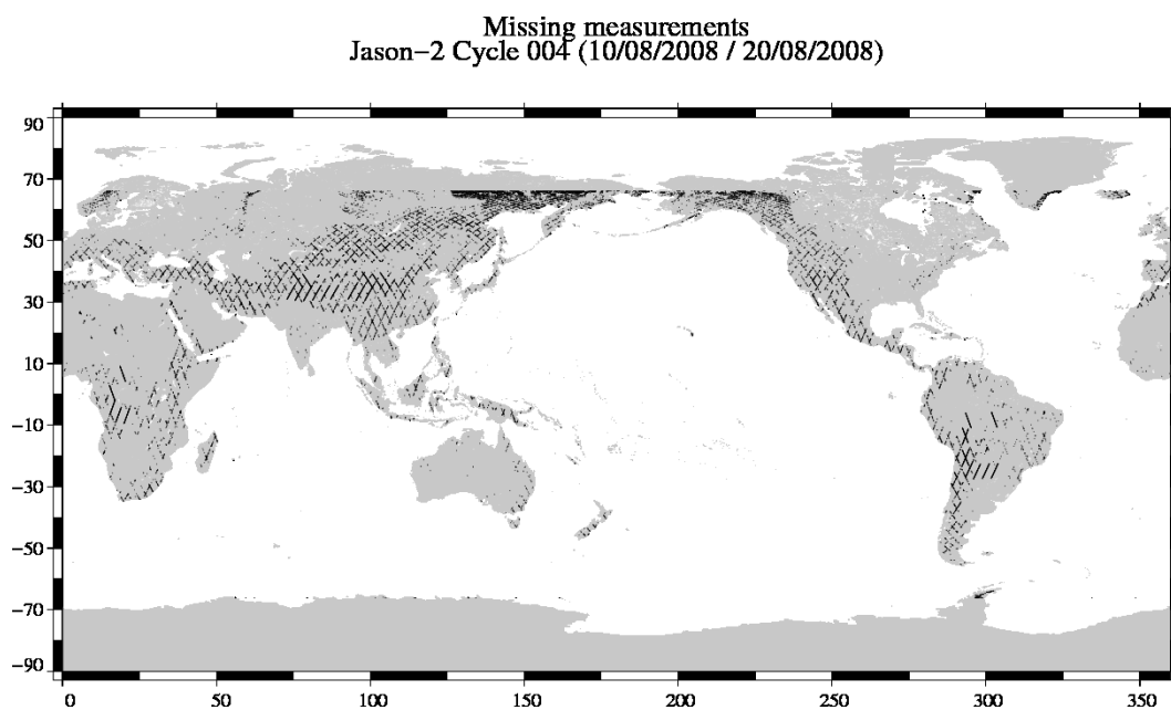
FIG. 1 – Missing measurements for cycle 004.
