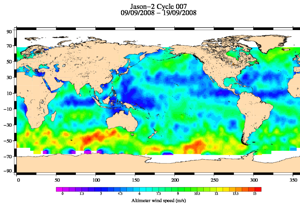
FIG. 9 – Altimeter wind speed for cycle 007.
