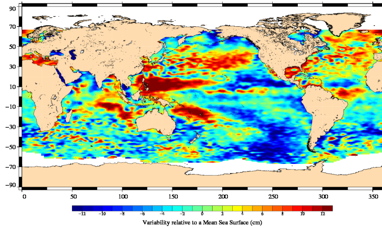
FIG. 18 – Sea level anomaly relative to MSS for cycle 007.
