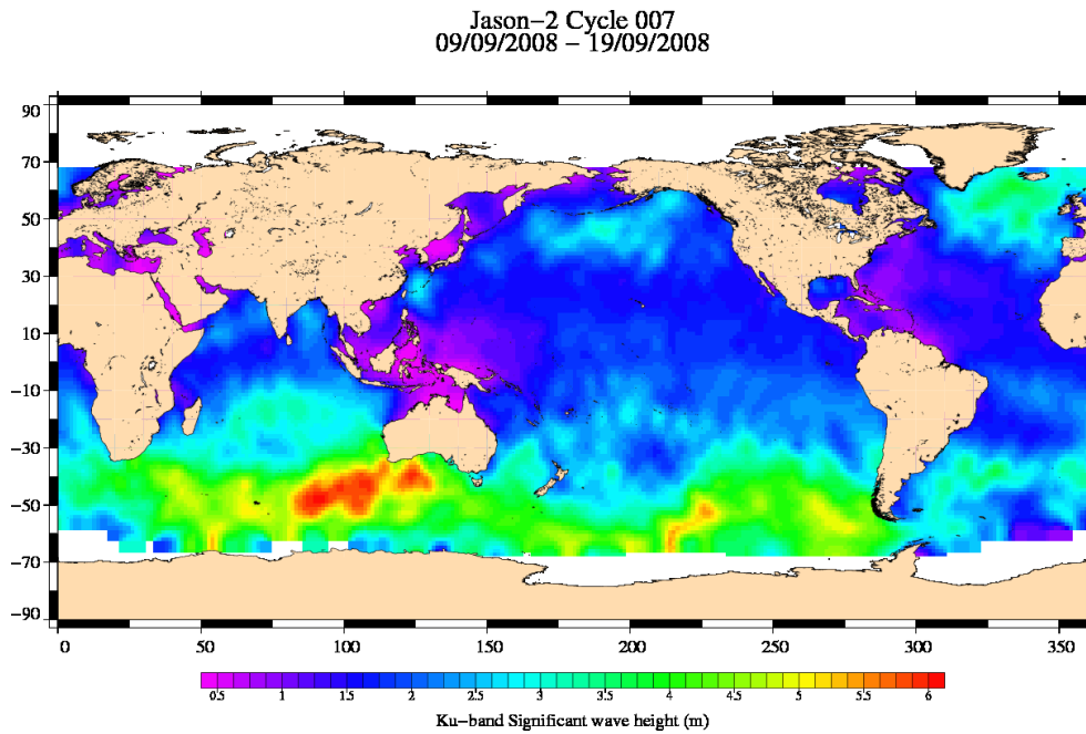
FIG. 5 – Significant wave height for cycle 007.
