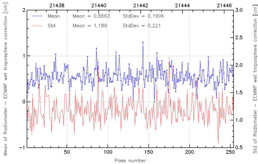
FIG. 11 – Pass monitoring of wet troposphere differences between radiometer and ECMWF model for Jason-2 cycle 007.
