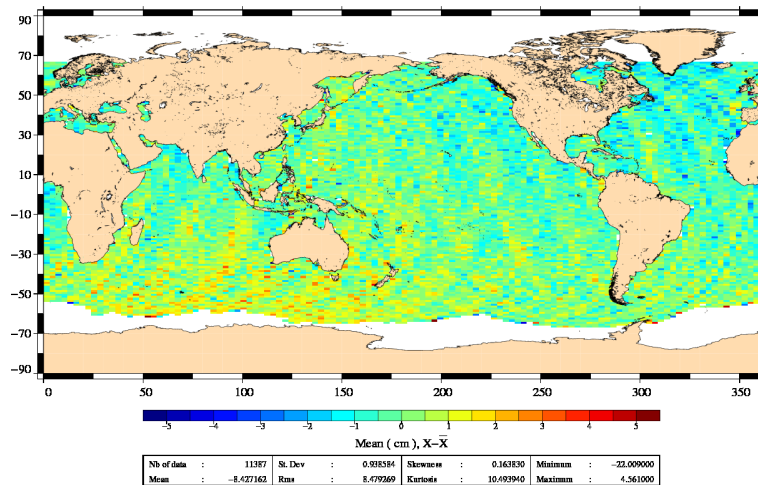
FIG. 20 – Jason-1 – Jason-2 SLA differences (without corrections) for cycle 007.
