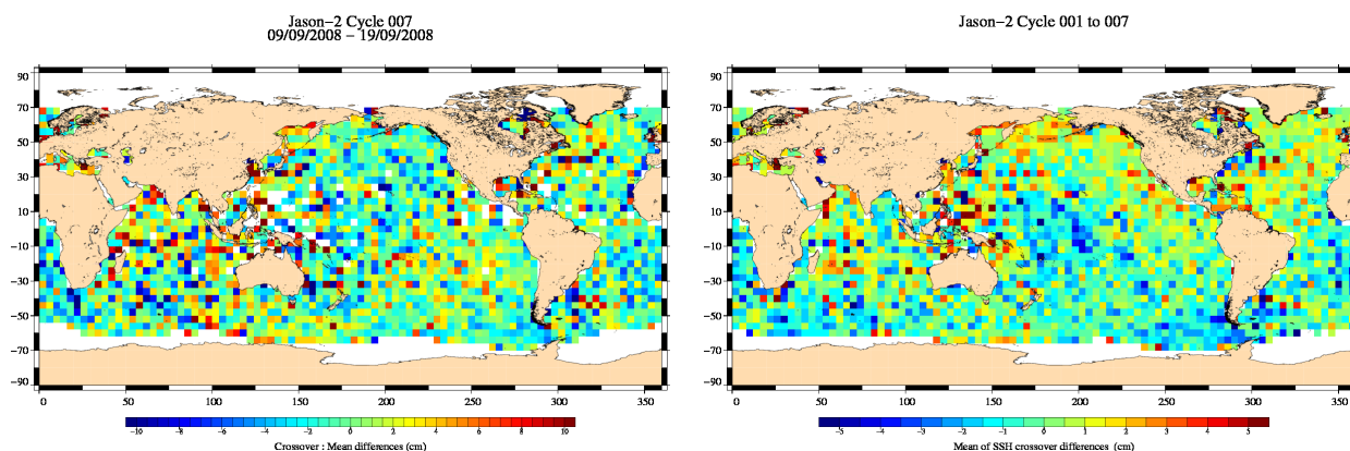
FIG. 13 – Mean SSH at crossovers for cycle 007 (left) and over the whole Jason-2 period (right).
