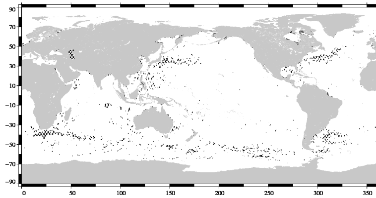
FIG. 19 – Differences higher than a 30 cm threshold for cycle 007.
