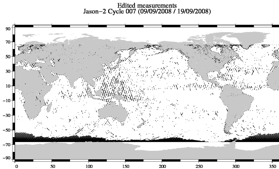
FIG. 2 – Edited measurements for cycle 007.
