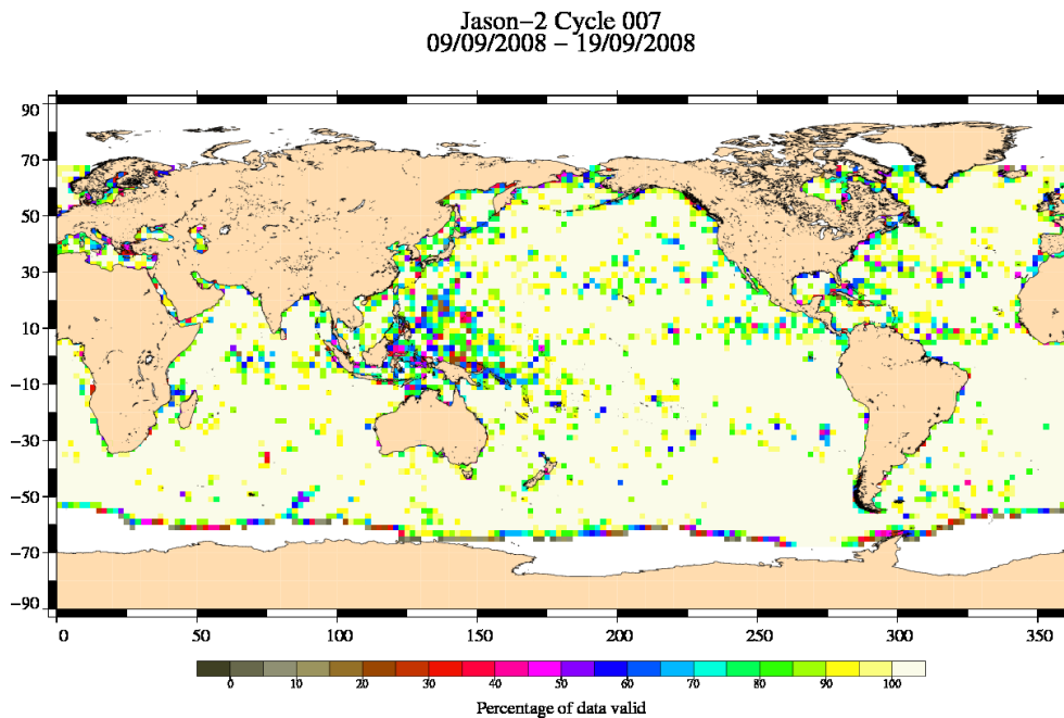
FIG. 3 – Percentage of valid measurements for cycle 007.
