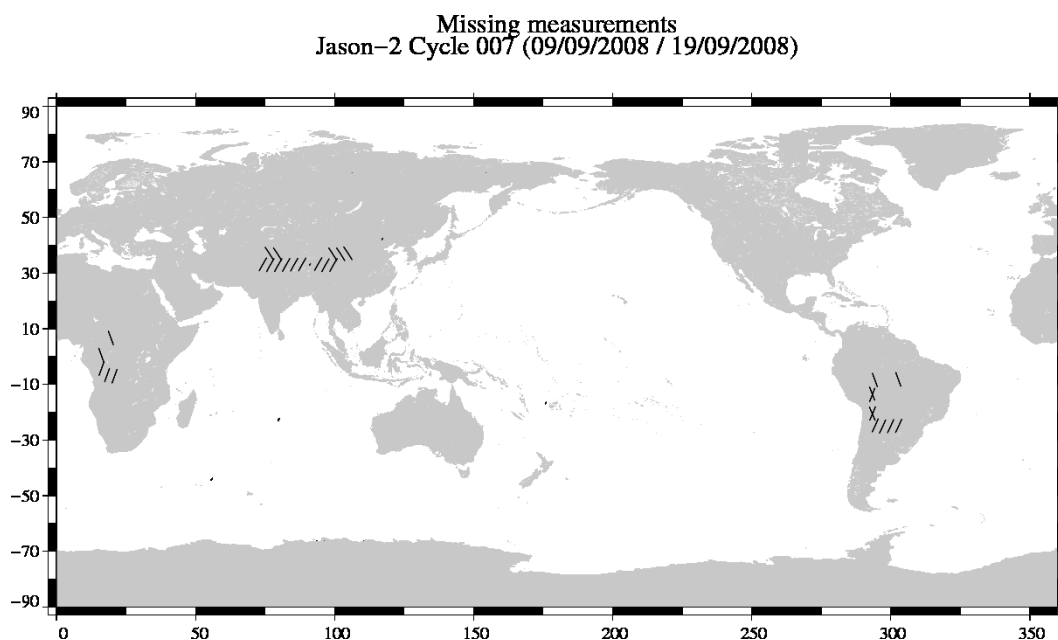
FIG. 1 – Missing measurements for cycle 007.
