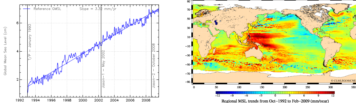
FIG. 22 – Global (left) and regional (right) MSL trends from 1993 onwards.
