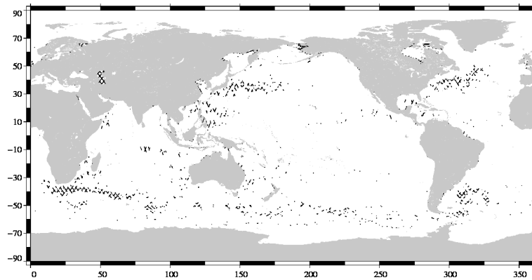
FIG. 19 – Differences higher than a 30 cm threshold for cycle 009.
