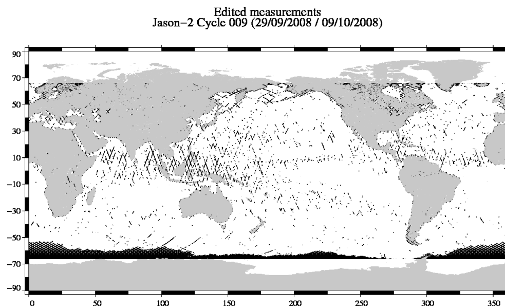
FIG. 2 – Edited measurements for cycle 009.
