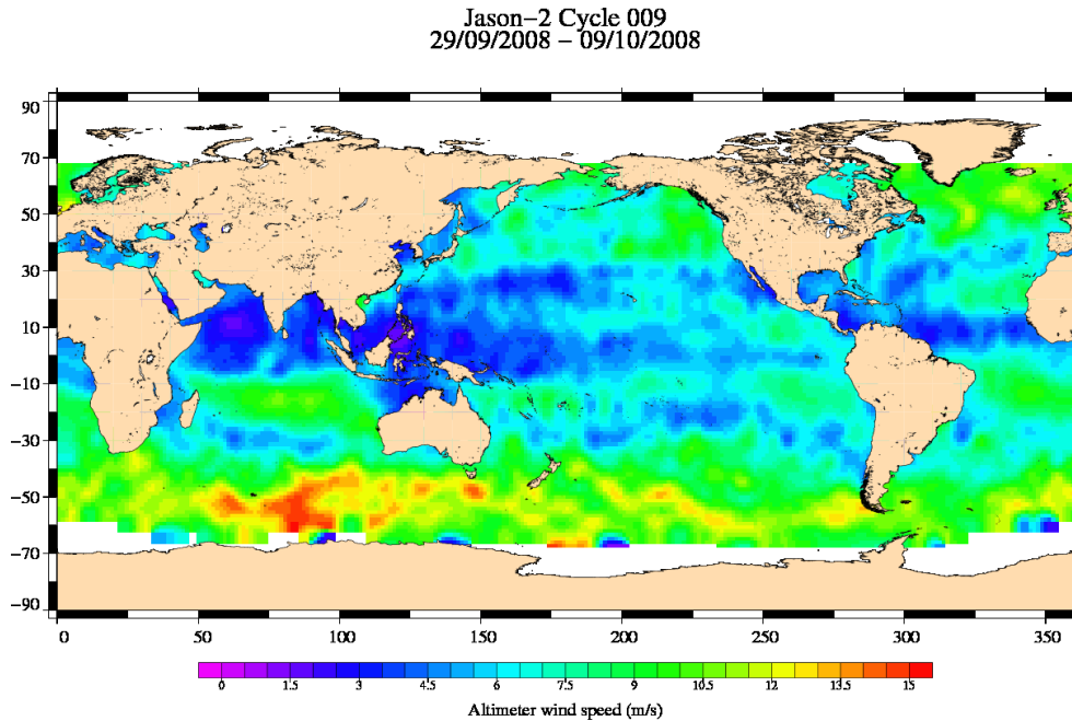
FIG. 9 – Altimeter wind speed for cycle 009.
