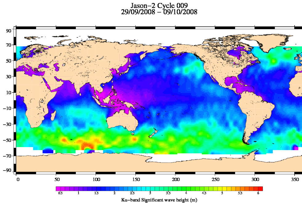
FIG. 5 – Significant wave height for cycle 009.
