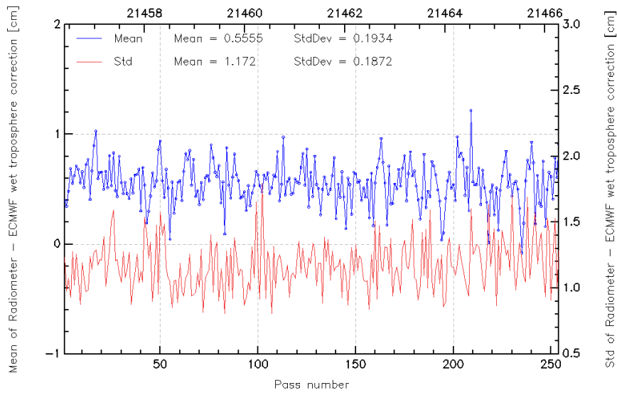
FIG. 11 – Pass monitoring of wet troposphere differences between radiometer and ECMWF model for Jason-2 cycle 009.
