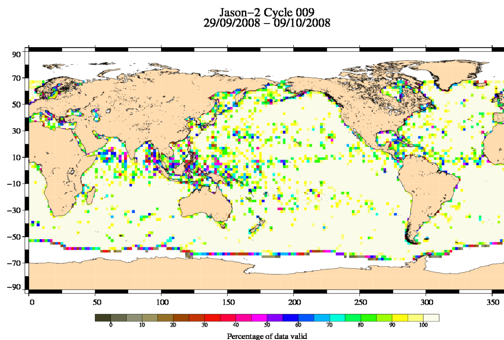
FIG. 3 – Percentage of valid measurements for cycle 009.
