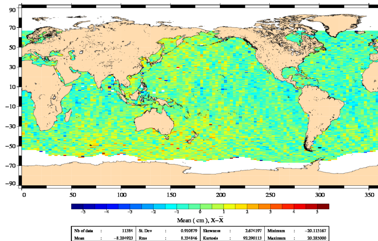
FIG. 20 – Jason-1 – Jason-2 SLA differences (without corrections) for cycle 009.
