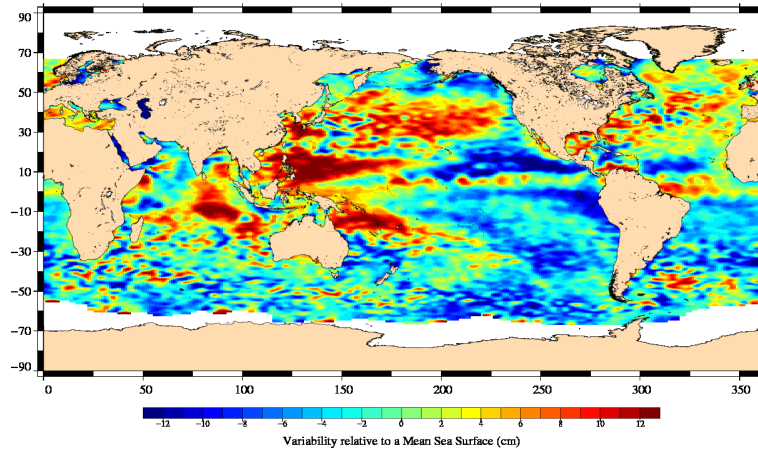
FIG. 18 – Sea level anomaly relative to MSS for cycle 009.
