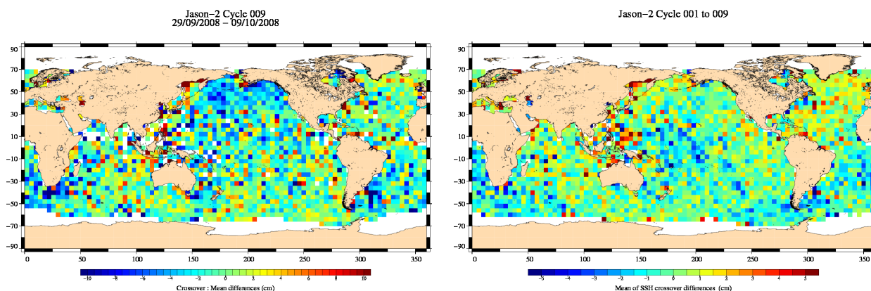
FIG. 13 – Mean SSH at crossovers for cycle 009 (left) and over the whole Jason-2 period (right).
