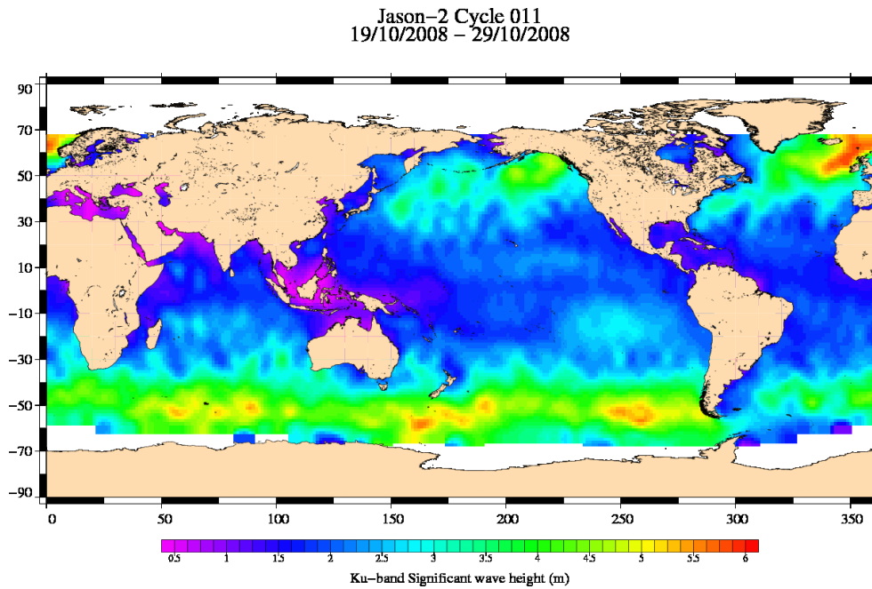
FIG. 6 – Significant wave height for cycle 011.
