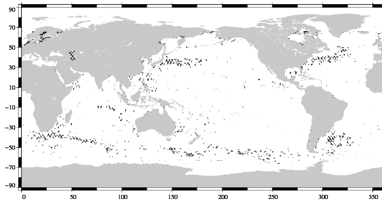
FIG. 20 – Differences higher than a 30 cm threshold for cycle 011.
