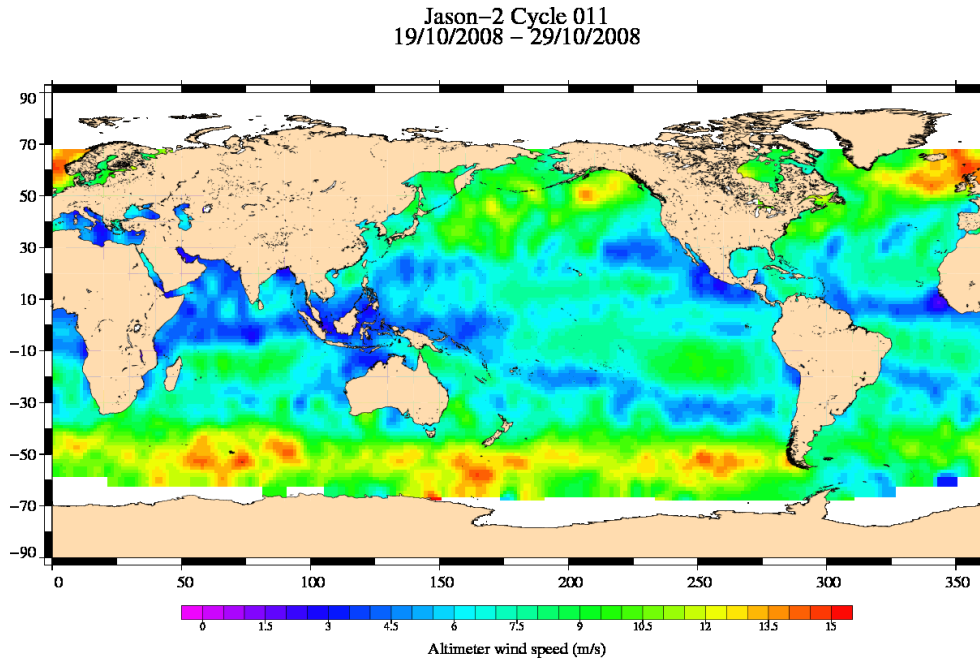
FIG. 10 – Altimeter wind speed for cycle 011.
