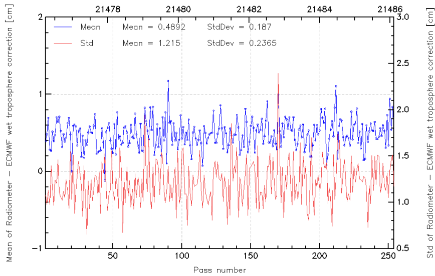
FIG. 12 – Pass monitoring of wet troposphere differences between radiometer and ECMWF model for Jason-2 cycle 011.
