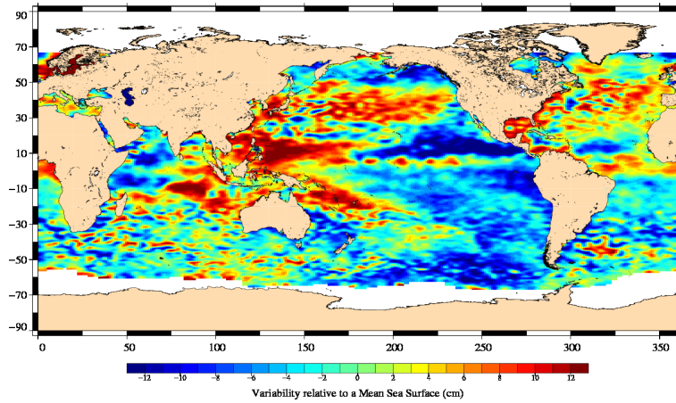
FIG. 19 – Sea level anomaly relative to MSS for cycle 011.
