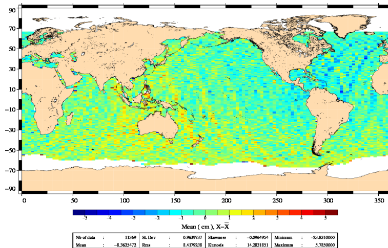
FIG. 21 – Jason-1 – Jason-2 SLA differences (without corrections) for cycle 011.
