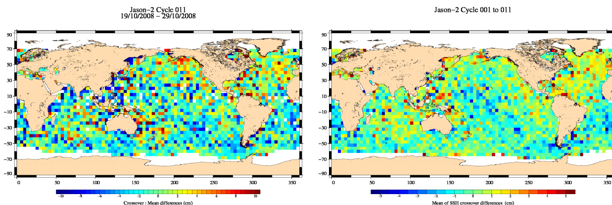
FIG. 14 – Mean SSH at crossovers for cycle 011 (left) and over the whole Jason-2 period (right).
