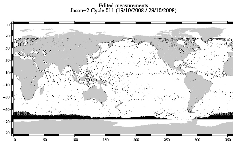
FIG. 2 – Edited measurements for cycle 011.
