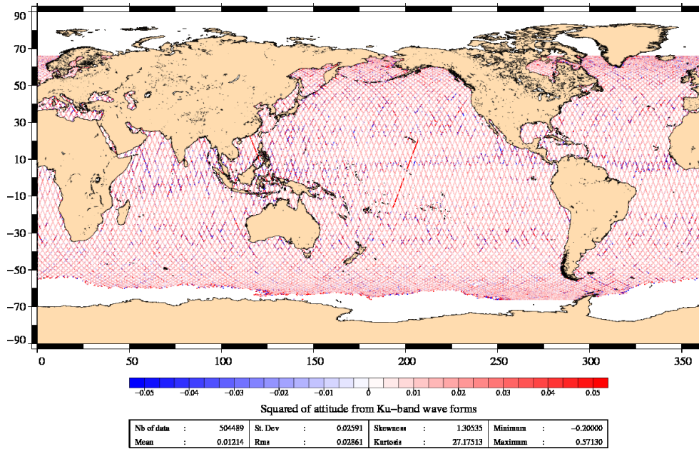
FIG. 4 – Apparent squared mispointing from waveforms for cycle 011.
