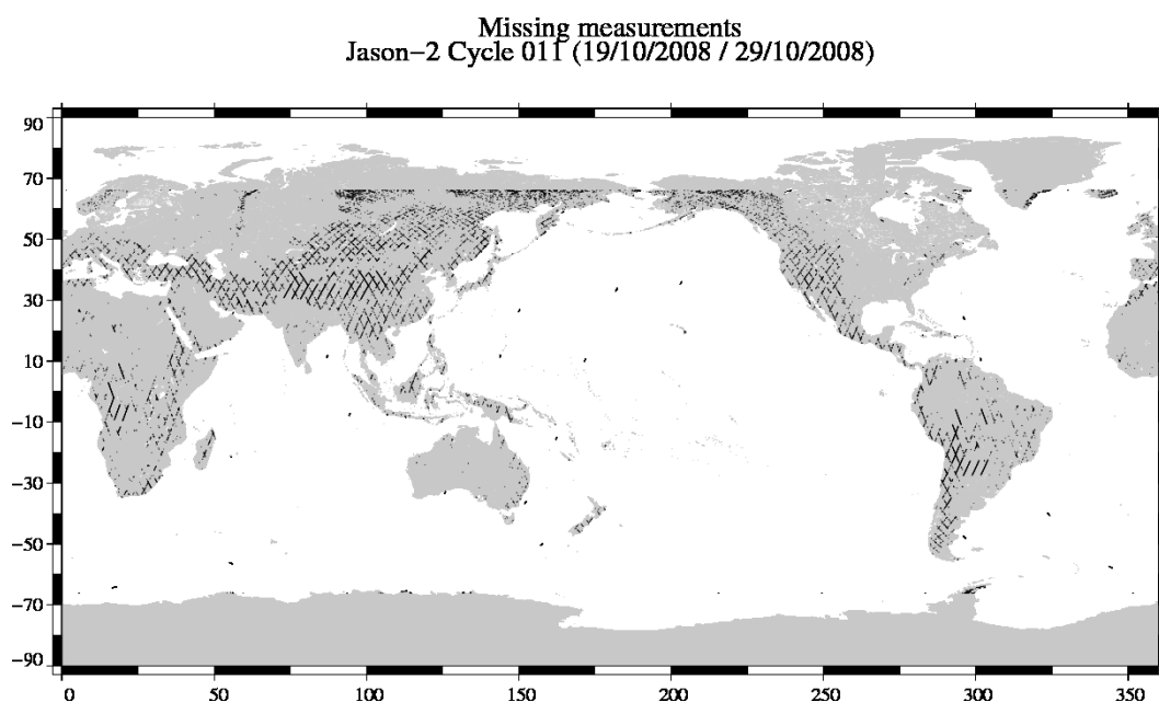
FIG. 1 – Missing measurements for cycle 011.
