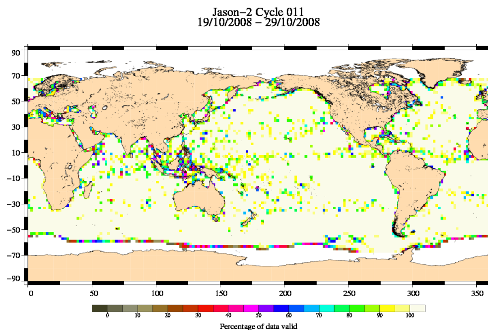
FIG. 3 – Percentage of valid measurements for cycle 011.
