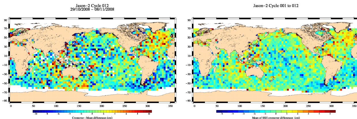
FIG. 13 – Mean SSH at crossovers for cycle 012 (left) and over the whole Jason-2 period (right).
