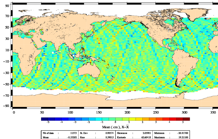
FIG. 20 – Jason-1 – Jason-2 SLA differences (without corrections) for cycle 012.
