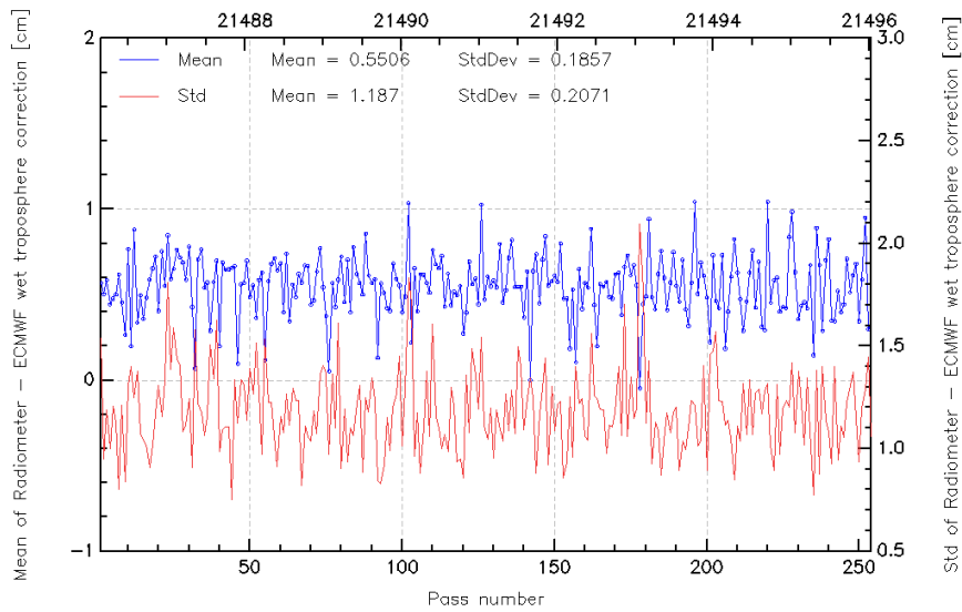
FIG. 11 – Pass monitoring of wet troposphere differences between radiometer and ECMWF model for Jason-2 cycle 012.
