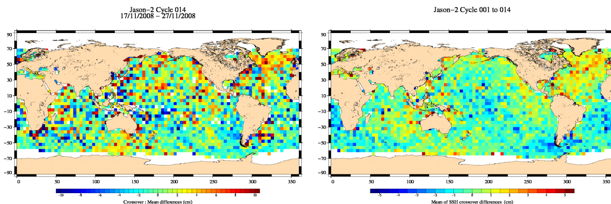
FIG. 13 – Mean SSH at crossovers for cycle 014 (left) and over the whole Jason-2 period (right).
