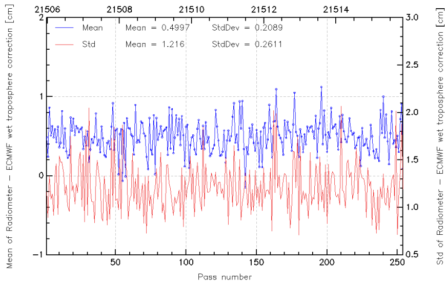
FIG. 11 – Pass monitoring of wet troposphere differences between radiometer and ECMWF model for Jason-2 cycle 014.
