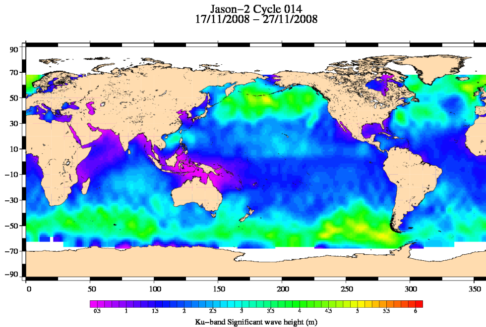
FIG. 5 – Significant wave height for cycle 014.
