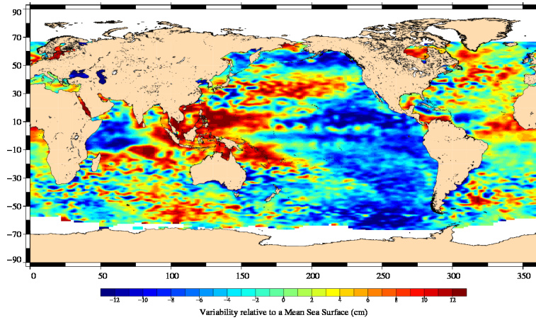
Jason-2 Cycle 014 17/11/2008 – 27/11/2008
