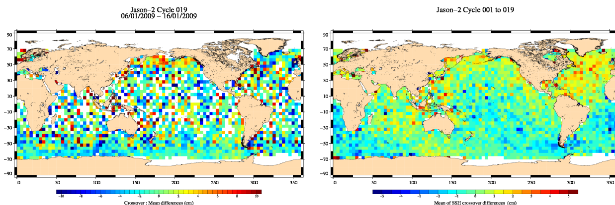
FIG. 13 – Mean SSH at crossovers for cycle 019 (left) and over the whole Jason-2 period (right).
