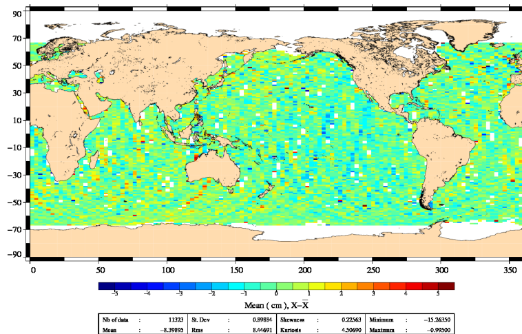
FIG. 20 – Jason-1 – Jason-2 SLA differences (without corrections) for cycle 019.
