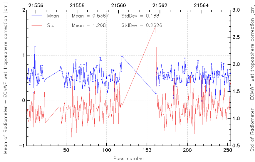
FIG. 11 – Pass monitoring of wet troposphere differences between radiometer and ECMWF model for Jason-2 cycle 019.
