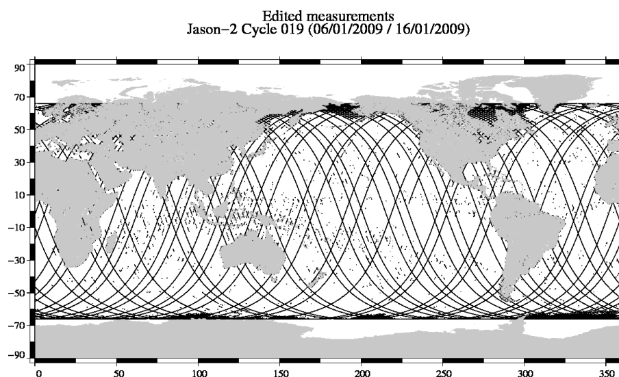
FIG. 2 – Edited measurements for cycle 019.
