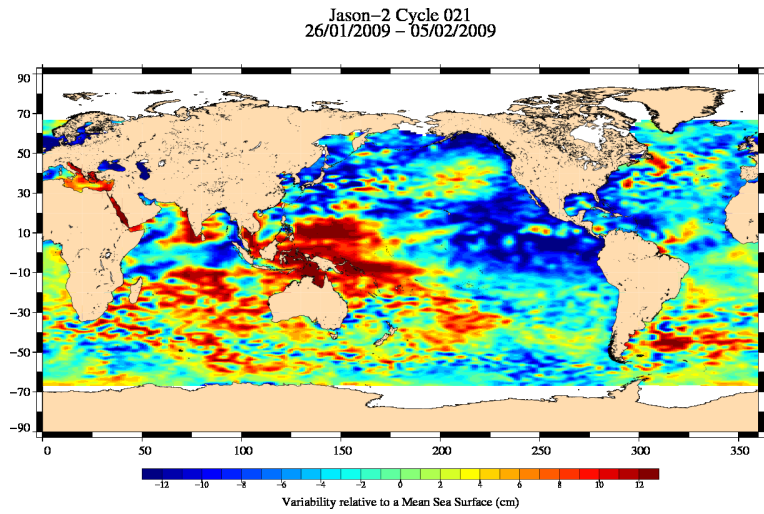
FIG. 18 – Sea level anomaly relative to MSS for cycle 021.
