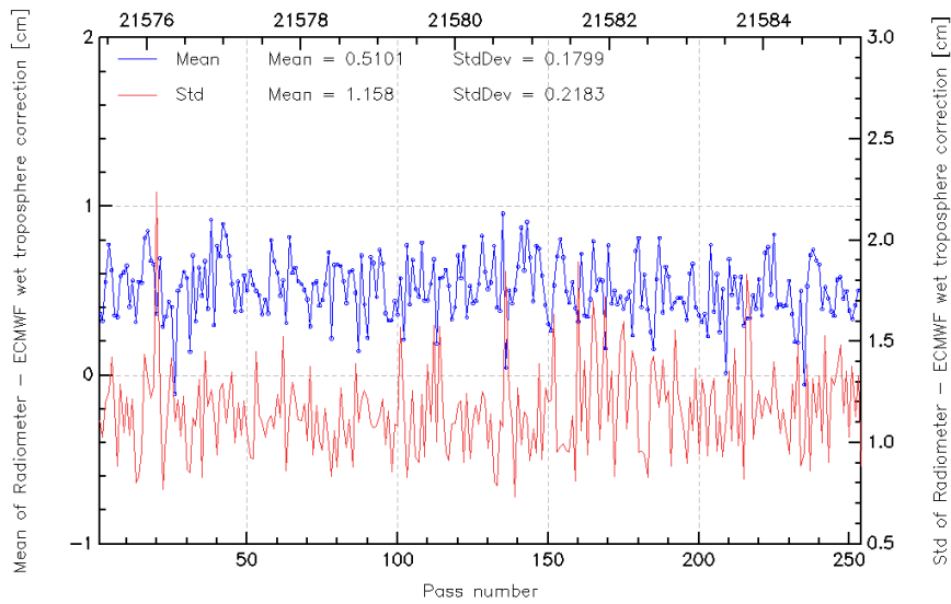
FIG. 11 – Pass monitoring of wet troposphere differences between radiometer and ECMWF model for Jason-2 cycle 021.
