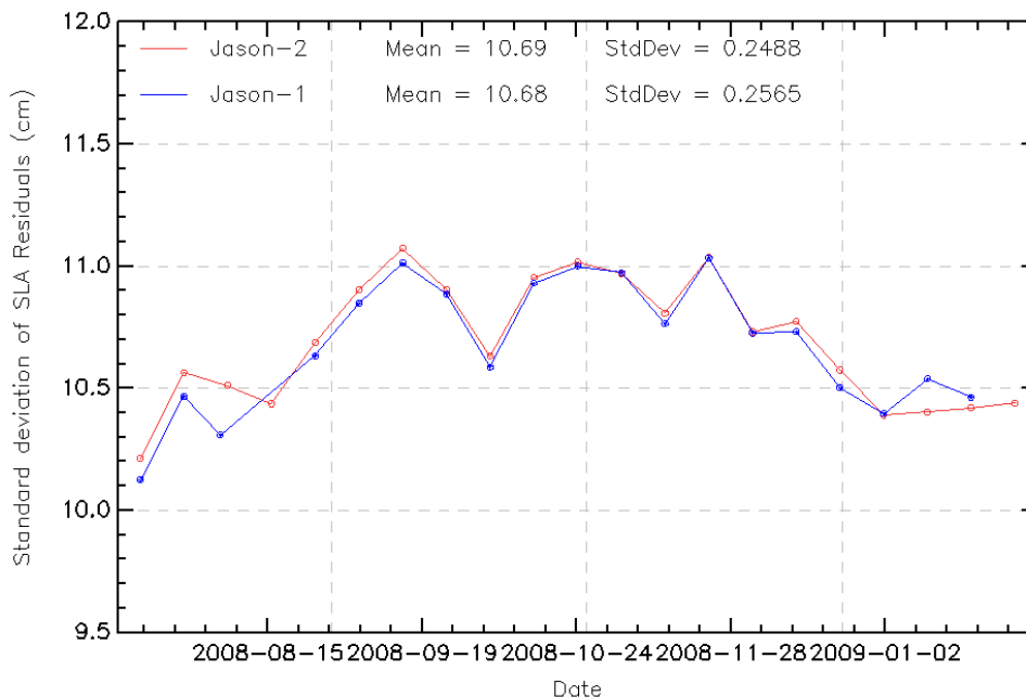
FIG. 20 – Cyclic monitoring standard deviation of along track SLA for Jason-1 and Jason-2.
