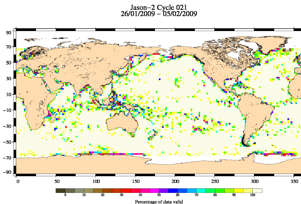
FIG. 3 – Percentage of valid measurements for cycle 021.
