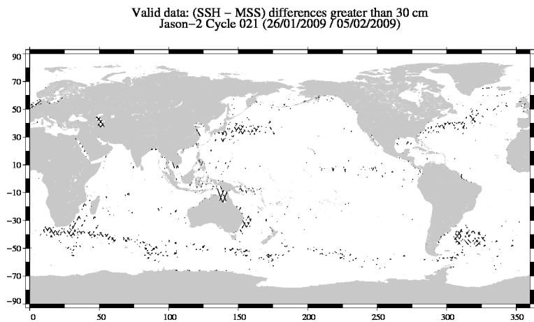
FIG. 19 – Differences higher than a 30 cm threshold for cycle 021.
