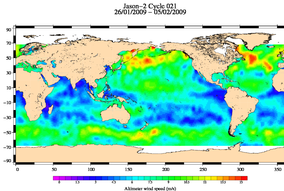
FIG. 9 – Altimeter wind speed for cycle 021.
