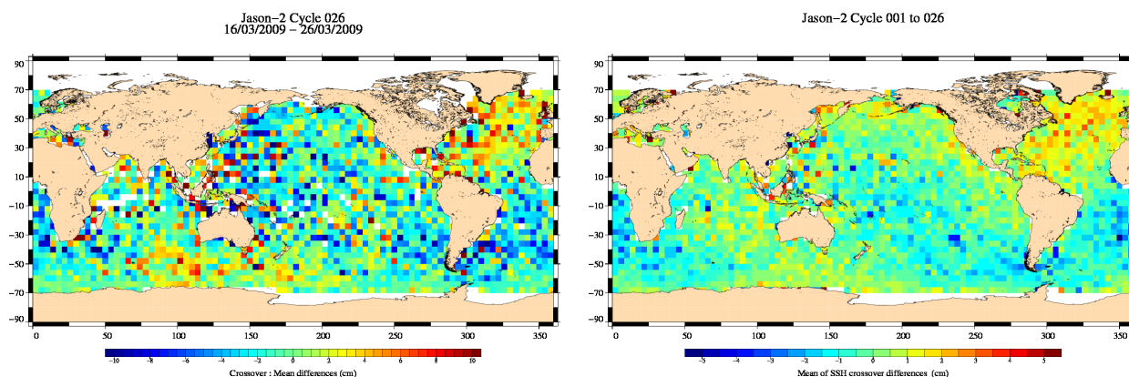
FIG. 13 – Mean SSH at crossovers for cycle 026 (left) and over the whole Jason-2 period (right).
