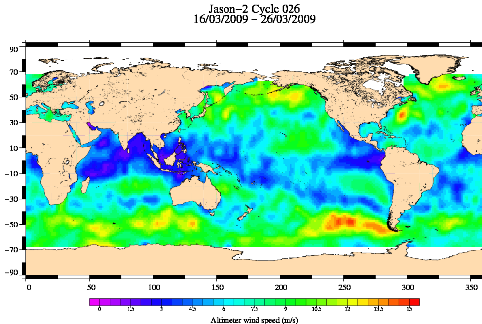
FIG. 9 – Altimeter wind speed for cycle 026.
