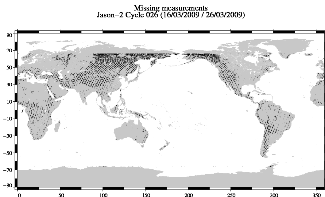
FIG. 1 – Missing measurements for cycle 026.
