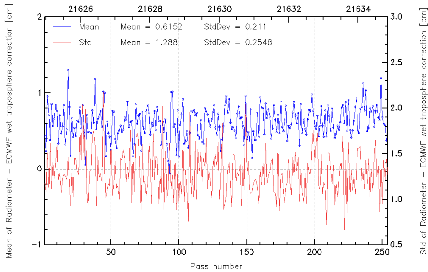
FIG. 11 – Pass monitoring of wet troposphere differences between radiometer and ECMWF model for Jason-2 cycle 026.
