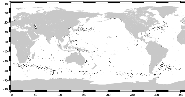
FIG. 19 – Differences higher than a 30 cm threshold for cycle 026.
