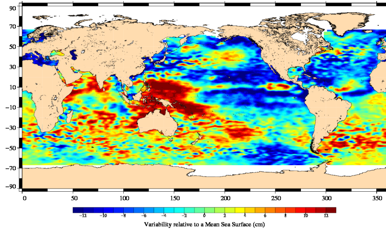
FIG. 18 – Sea level anomaly relative to MSS for cycle 026.
