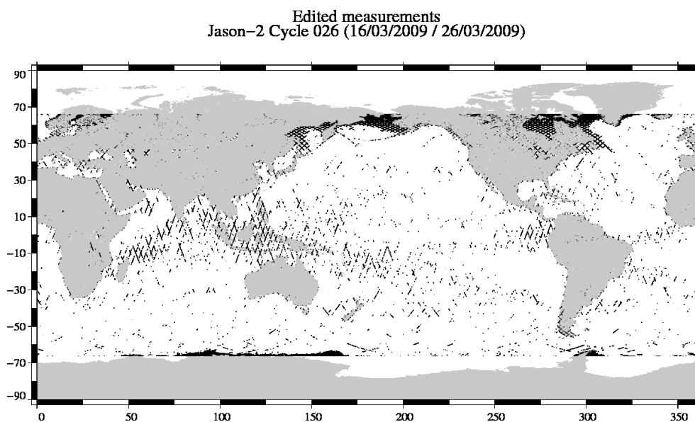
FIG. 2 – Edited measurements for cycle 026.
