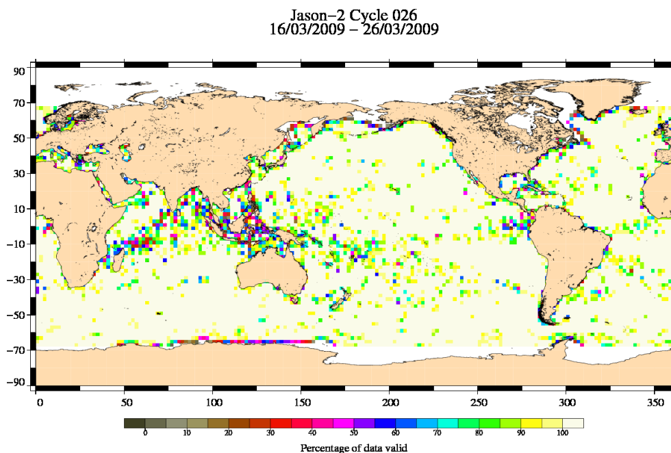
FIG. 3 – Percentage of valid measurements for cycle 026.
