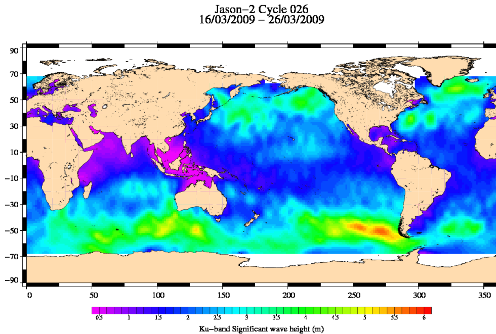
FIG. 5 – Significant wave height for cycle 026.
