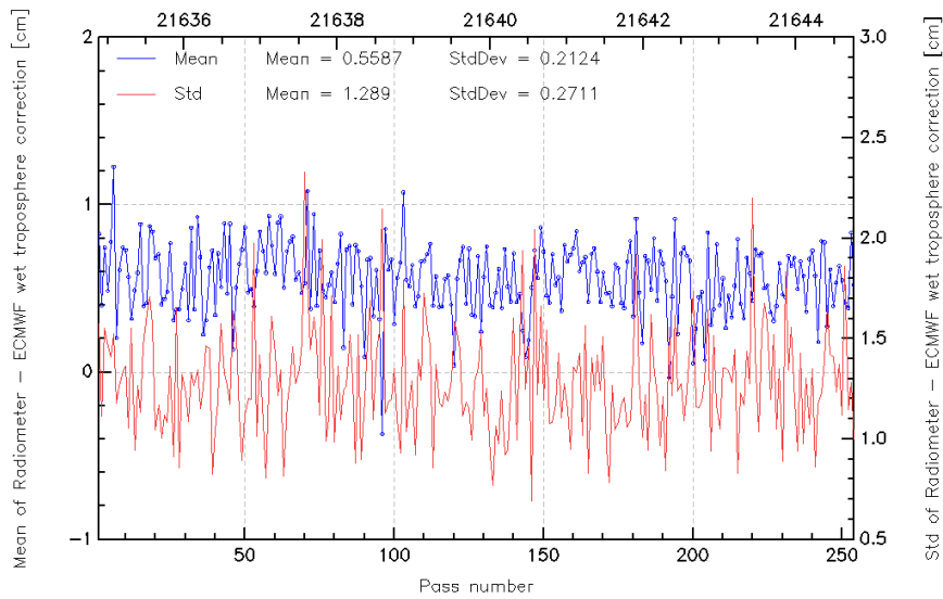
FIG. 11 – Pass monitoring of wet troposphere differences between radiometer and ECMWF model for Jason-2 cycle 027.
