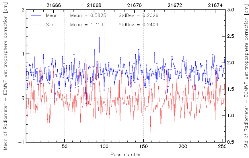
FIG. 11 – Pass monitoring of wet troposphere differences between radiometer and ECMWF model for Jason-2 cycle 030.
