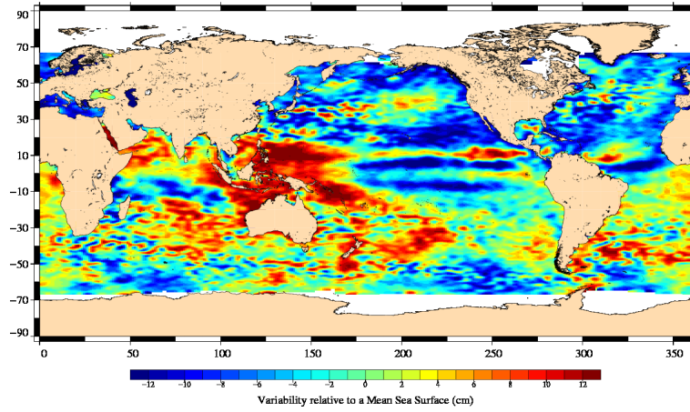
FIG. 18 – Sea level anomaly relative to MSS for cycle 030.
