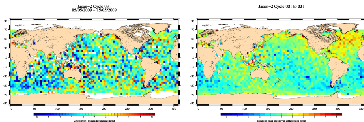
FIG. 13 – Mean SSH at crossovers for cycle 031 (left) and over the whole Jason-2 period (right).
