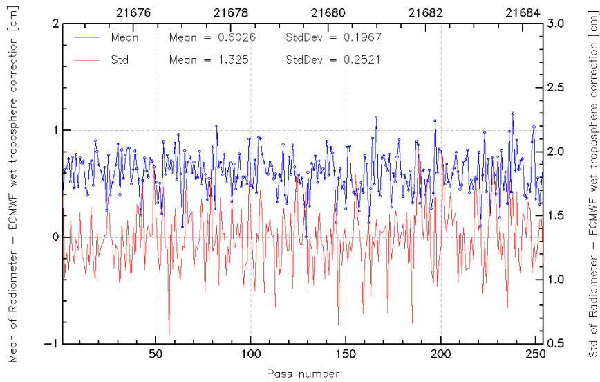
FIG. 11 – Pass monitoring of wet troposphere differences between radiometer and ECMWF model for Jason-2 cycle 031.
