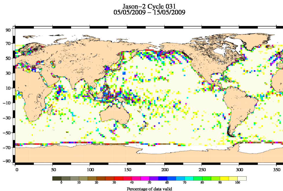
FIG. 3 – Percentage of valid measurements for cycle 031.
