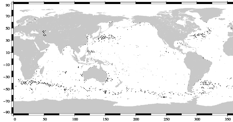
FIG. 19 – Differences higher than a 30 cm threshold for cycle 031.
