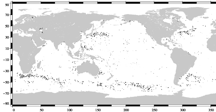
FIG. 19 – Differences higher than a 30 cm threshold for cycle 033.
