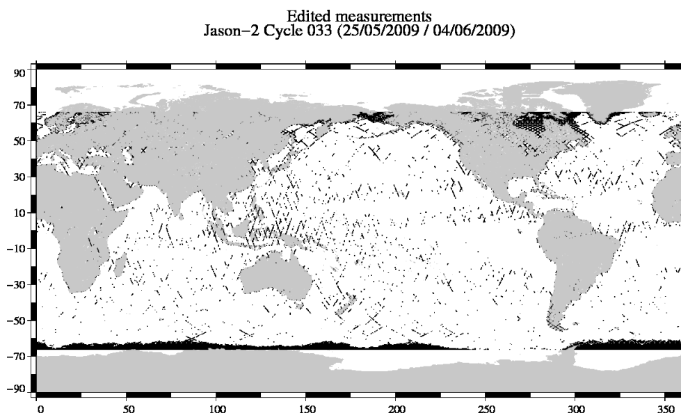
FIG. 2 – Edited measurements for cycle 033.
