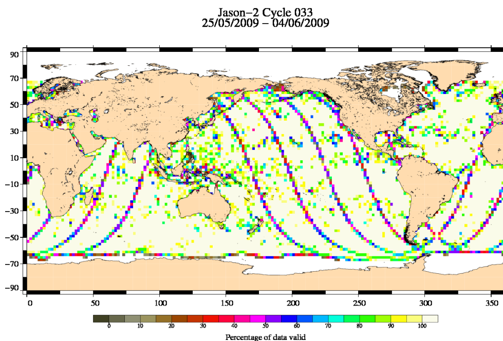
FIG. 3 – Percentage of valid measurements for cycle 033.
