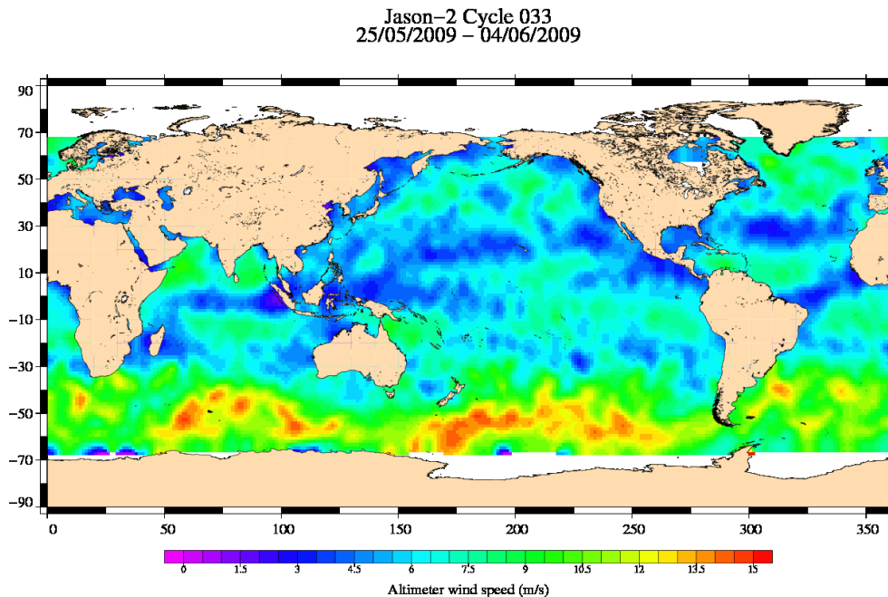
FIG. 9 – Altimeter wind speed for cycle 033.
