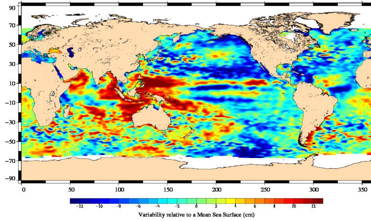
FIG. 18 – Sea level anomaly relative to MSS for cycle 033.
