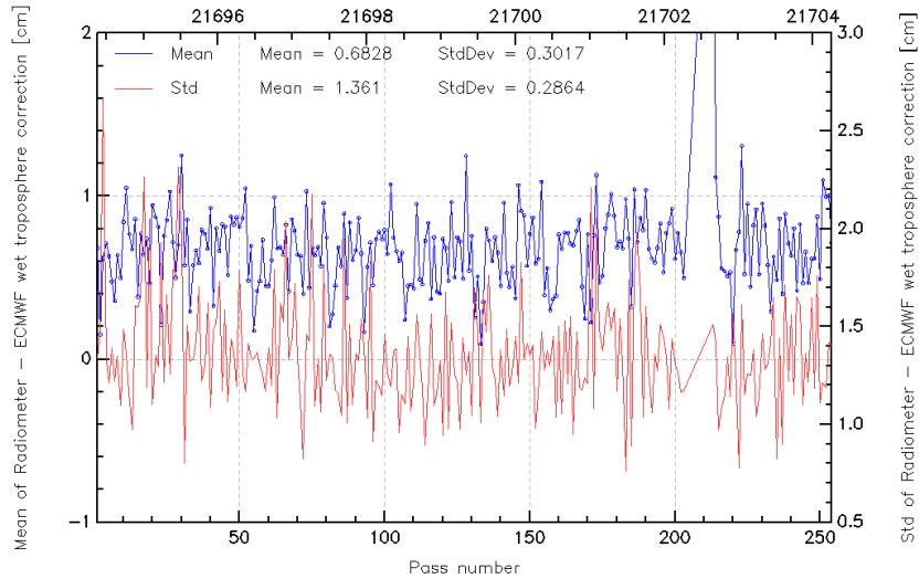
FIG. 11 – Pass monitoring of wet troposphere differences between radiometer and ECMWF model for Jason-2 cycle 033.
