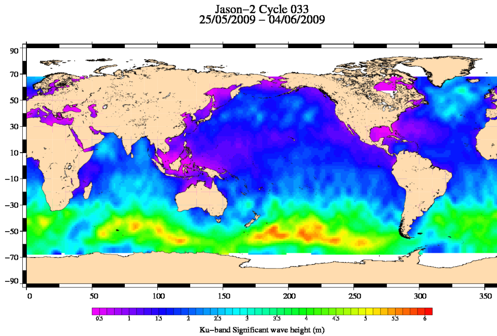
FIG. 5 – Significant wave height for cycle 033.
