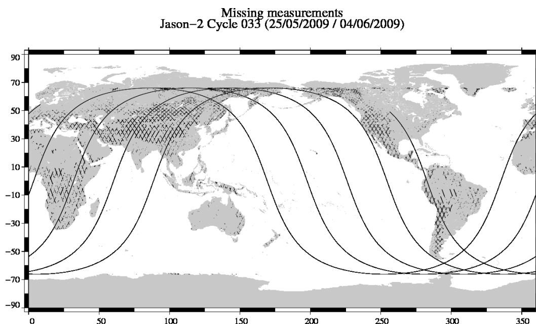
FIG. 1 – Missing measurements for cycle 033.
