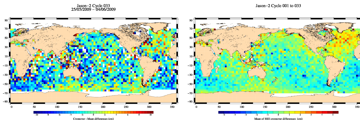
FIG. 13 – Mean SSH at crossovers for cycle 033 (left) and over the whole Jason-2 period (right).
