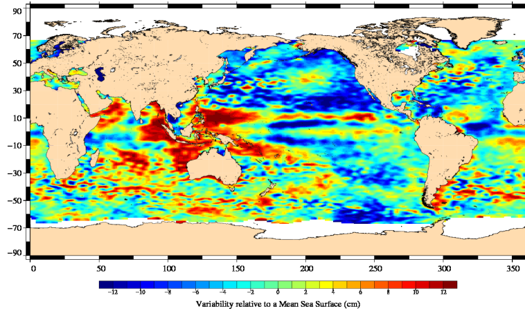
FIG. 18 – Sea level anomaly relative to MSS for cycle 034.
