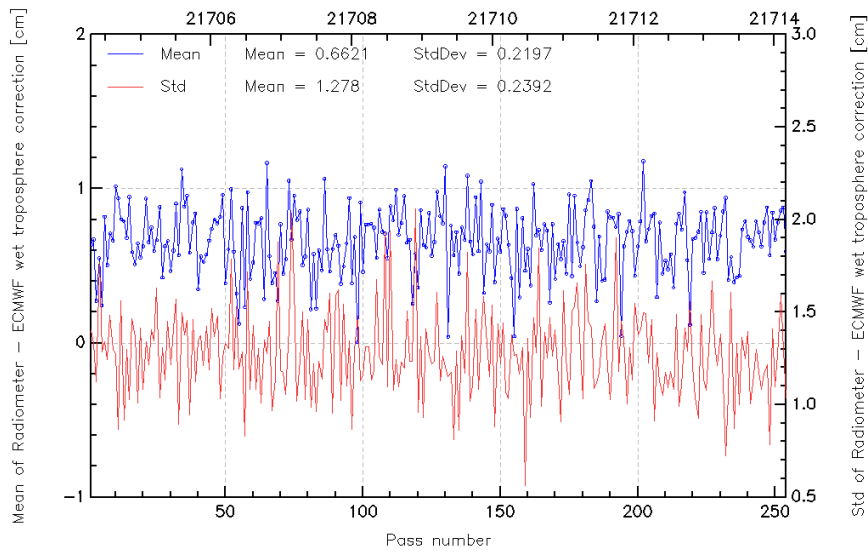
FIG. 11 – Pass monitoring of wet troposphere differences between radiometer and ECMWF model for Jason-2 cycle 034.
