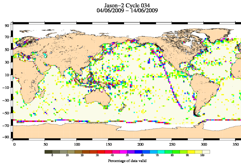
FIG. 3 – Percentage of valid measurements for cycle 034.
