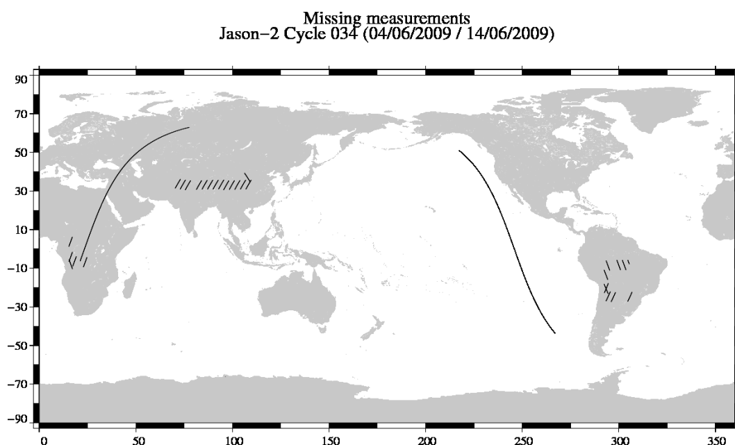
FIG. 1 – Missing measurements for cycle 034.
