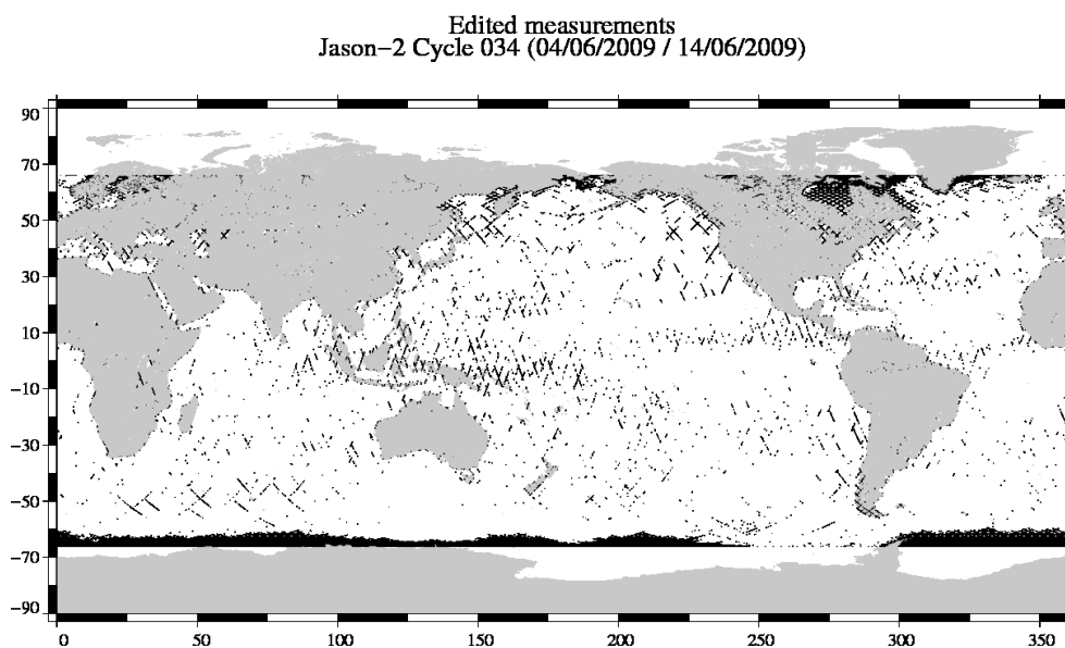
FIG. 2 – Edited measurements for cycle 034.
