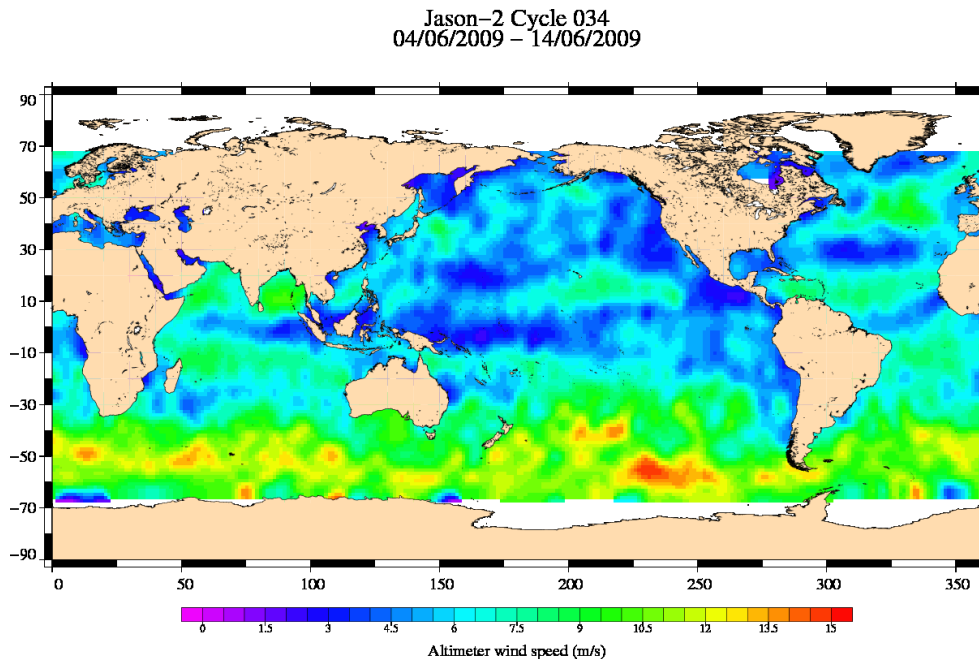
FIG. 9 – Altimeter wind speed for cycle 034.
