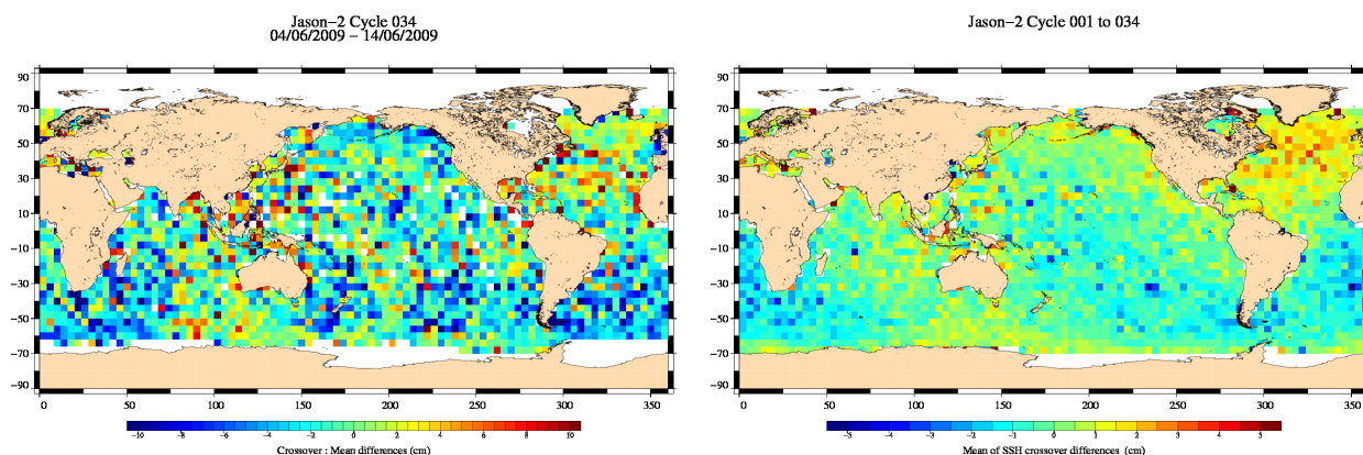
FIG. 13 – Mean SSH at crossovers for cycle 034 (left) and over the whole Jason-2 period (right).
