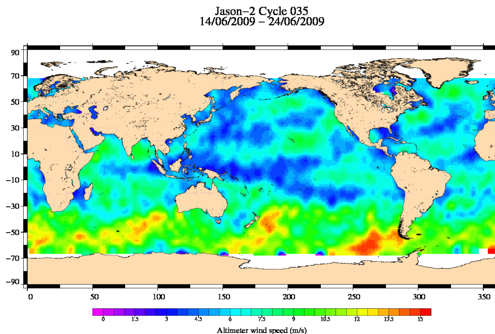
FIG. 9 – Altimeter wind speed for cycle 035.
