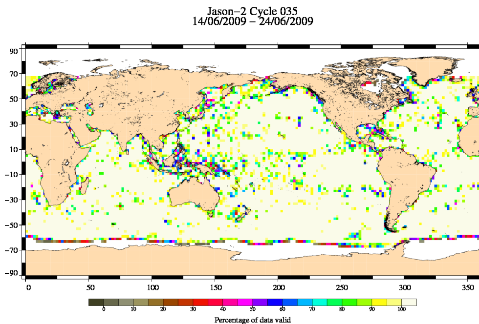
FIG. 3 – Percentage of valid measurements for cycle 035.
