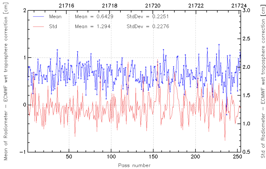
FIG. 11 – Pass monitoring of wet troposphere differences between radiometer and ECMWF model for Jason-2 cycle 035.
