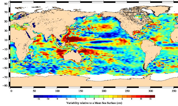
FIG. 18 – Sea level anomaly relative to MSS for cycle 037.
