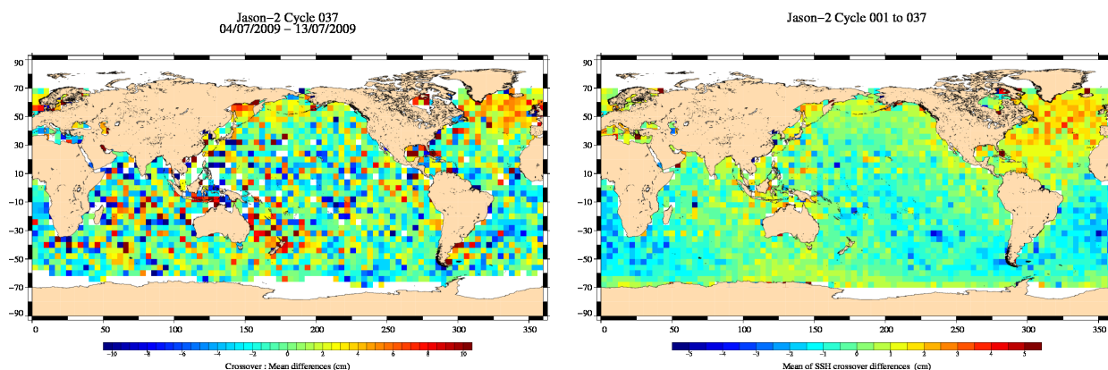
FIG. 13 – Mean SSH at crossovers for cycle 037 (left) and over the whole Jason-2 period (right).
