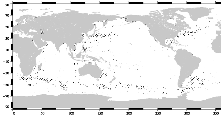
FIG. 19 – Differences higher than a 30 cm threshold for cycle 037.
