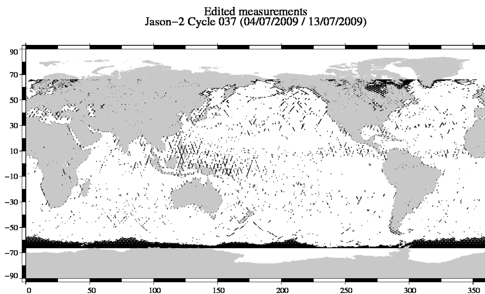
FIG. 2 – Edited measurements for cycle 037.
