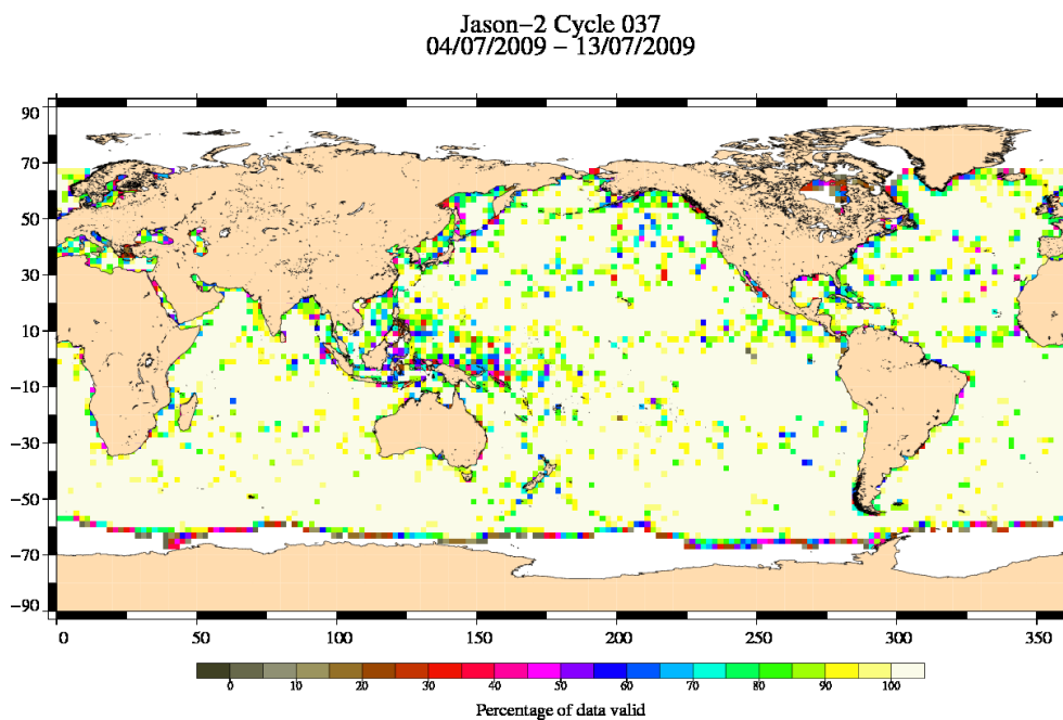
FIG. 3 – Percentage of valid measurements for cycle 037.
