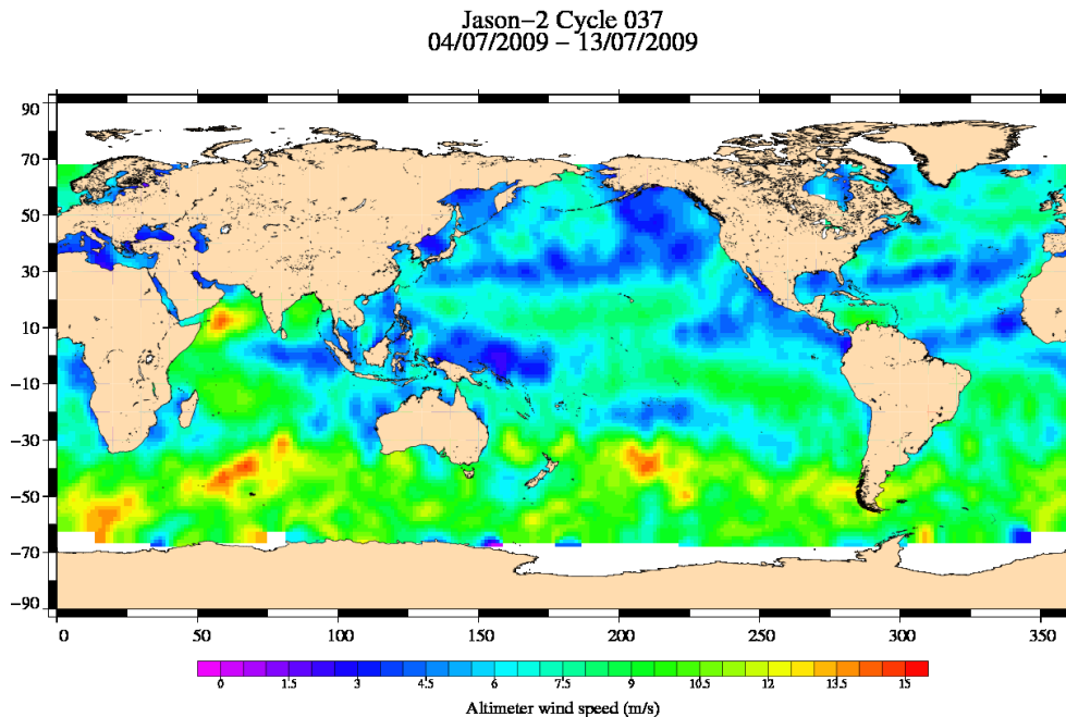
FIG. 9 – Altimeter wind speed for cycle 037.
