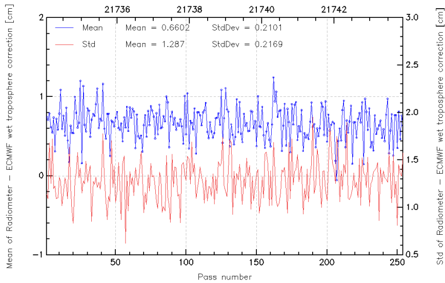
FIG. 11 – Pass monitoring of wet troposphere differences between radiometer and ECMWF model for Jason-2 cycle 037.
