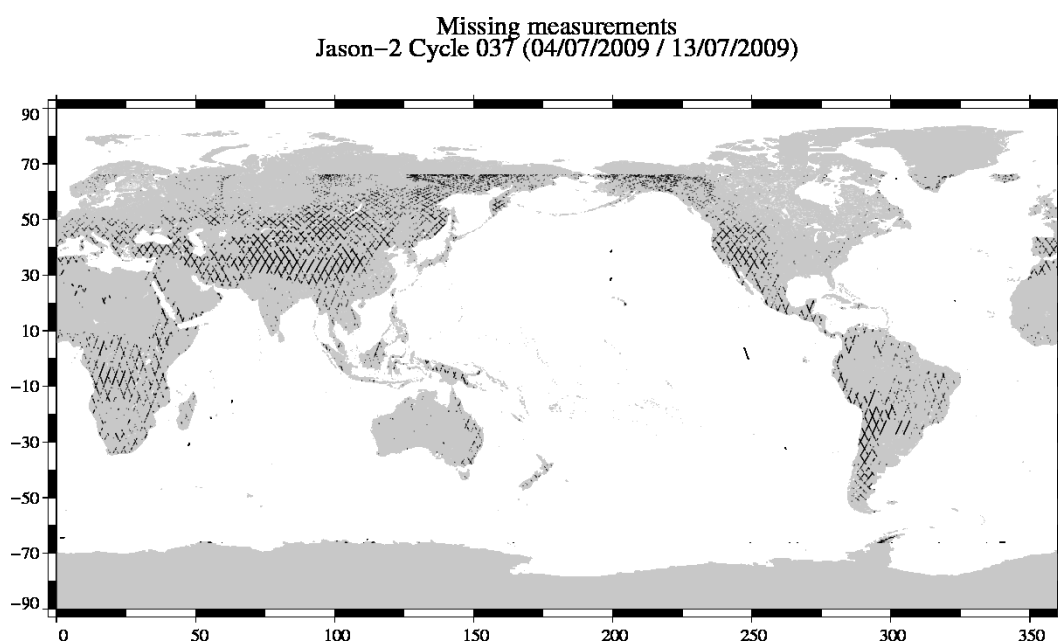
FIG. 1 – Missing measurements for cycle 037.
