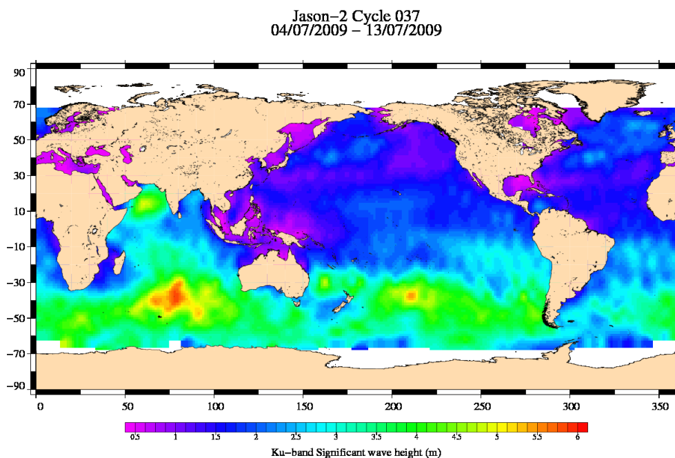
FIG. 5 – Significant wave height for cycle 037.
