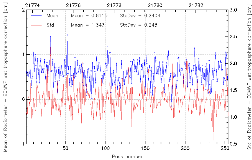
FIG. 11 – Pass monitoring of wet troposphere differences between radiometer and ECMWF model for Jason-2 cycle 041.
