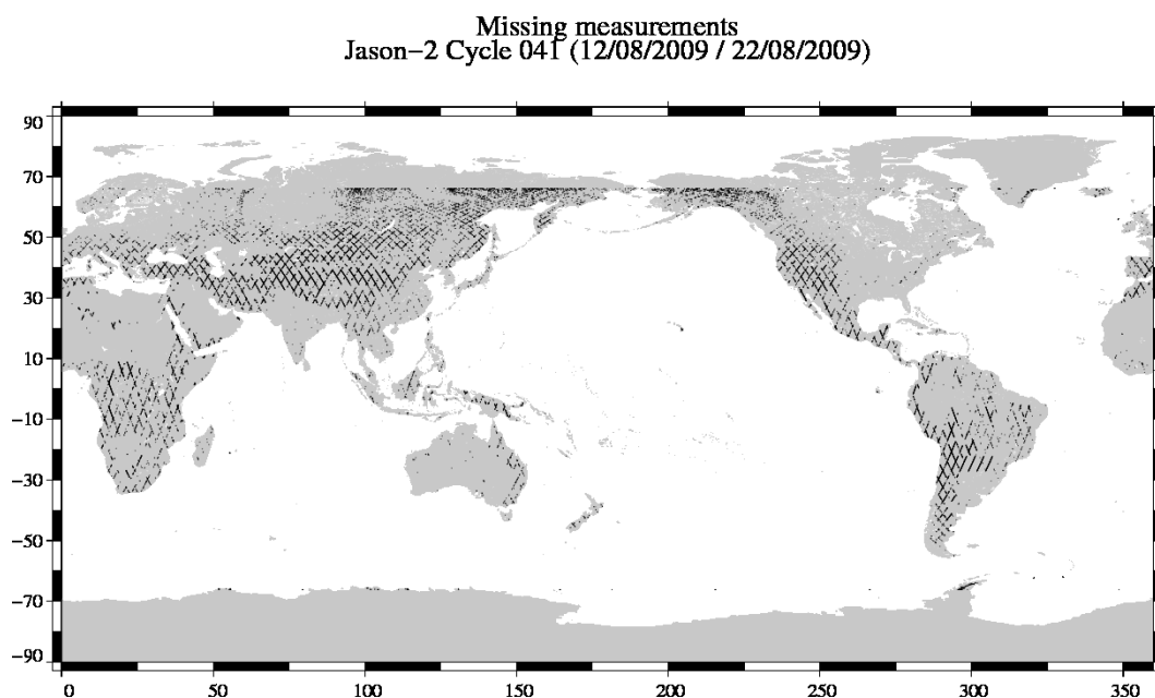
FIG. 1 – Missing measurements for cycle 041.
