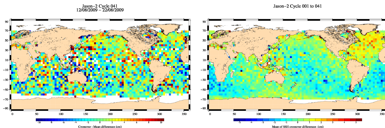
FIG. 13 – Mean SSH at crossovers for cycle 041 (left) and over the whole Jason-2 period (right).
