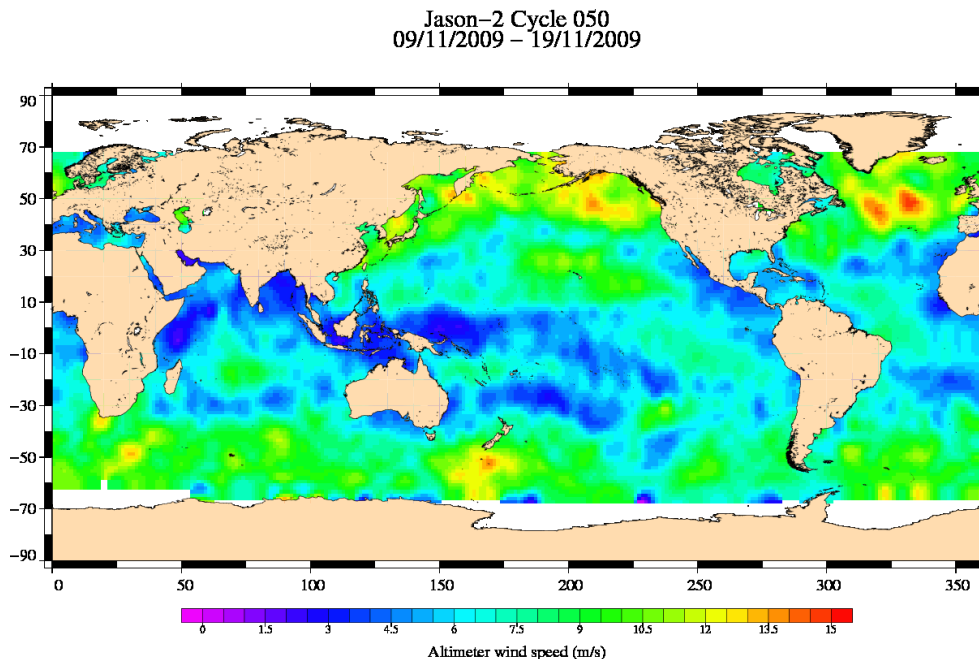
FIG. 9 – Altimeter wind speed for cycle 050.
