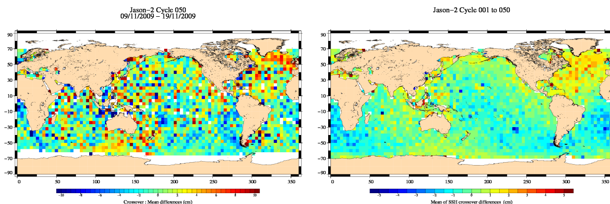
FIG. 13 – Mean SSH at crossovers for cycle 050 (left) and over the whole Jason-2 period (right).
