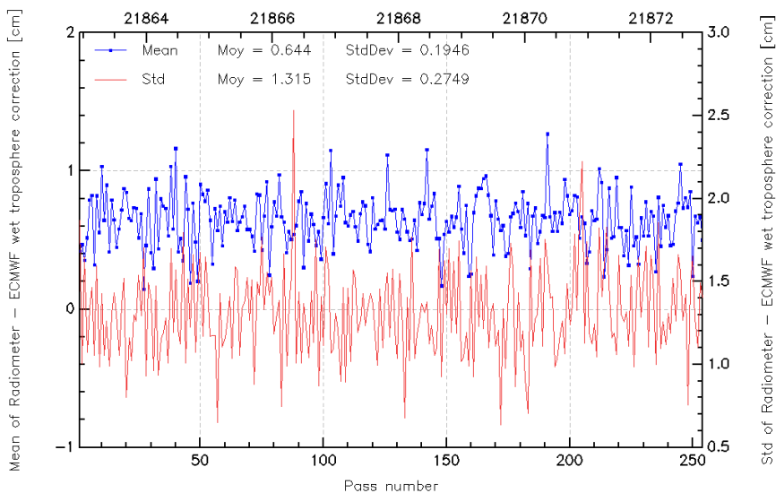
FIG. 11 – Pass monitoring of wet troposphere differences between radiometer and ECMWF model for Jason-2 cycle 050.
