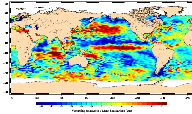
Jason-2 Cycle 050 09/11/2009 - 19/11/2009
