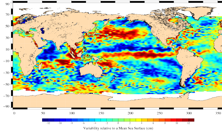
FIG. 18 – Sea level anomaly relative to MSS for cycle 051.
