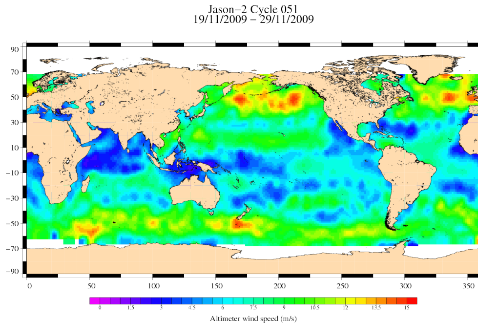
FIG. 9 – Altimeter wind speed for cycle 051.
