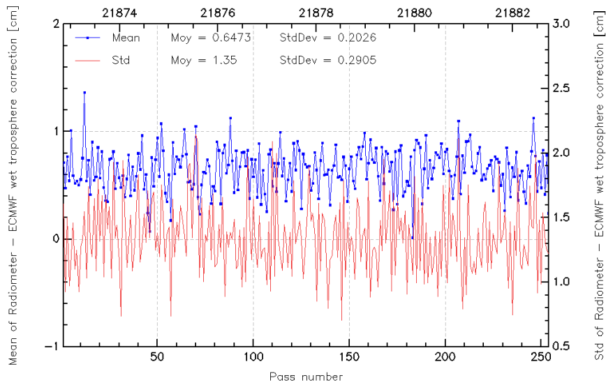
FIG. 11 – Pass monitoring of wet troposphere differences between radiometer and ECMWF model for Jason-2 cycle 051.
