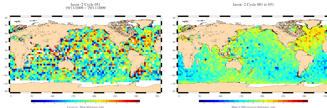
FIG. 13 – Mean SSH at crossovers for cycle 051 (left) and over the whole Jason-2 period (right).
