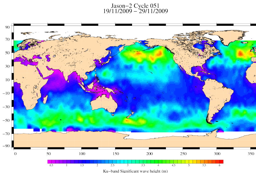
FIG. 5 – Significant wave height for cycle 051.
