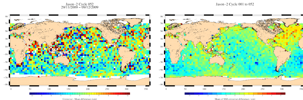
FIG. 13 – Mean SSH at crossovers for cycle 052 (left) and over the whole Jason-2 period (right).
