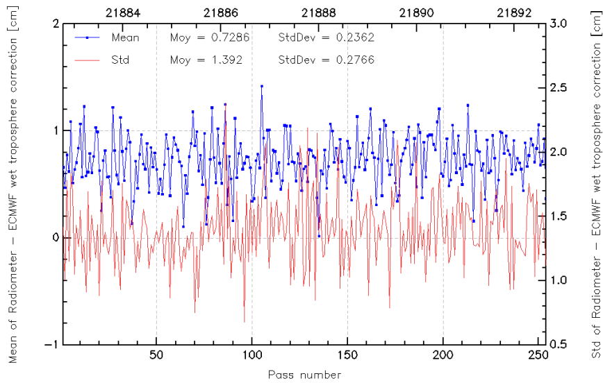
FIG. 11 – Pass monitoring of wet troposphere differences between radiometer and ECMWF model for Jason-2 cycle 052.
