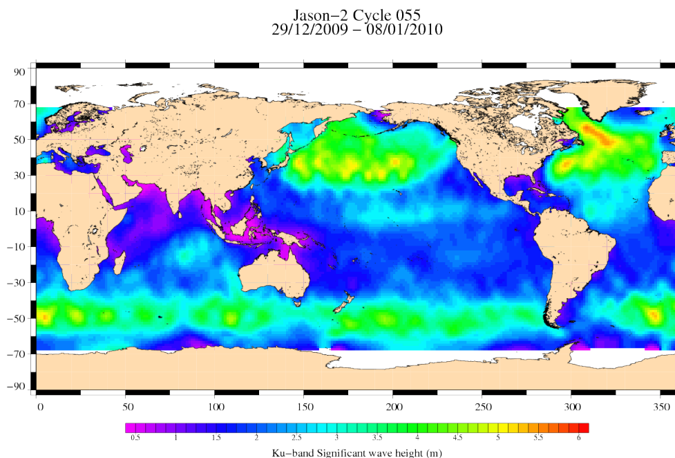
FIG. 5 – Significant wave height for cycle 055.
