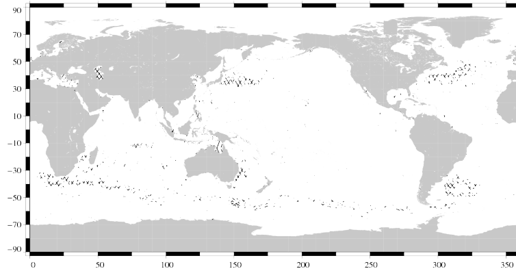
FIG. 19 – Differences higher than a 30 cm threshold for cycle 055.
