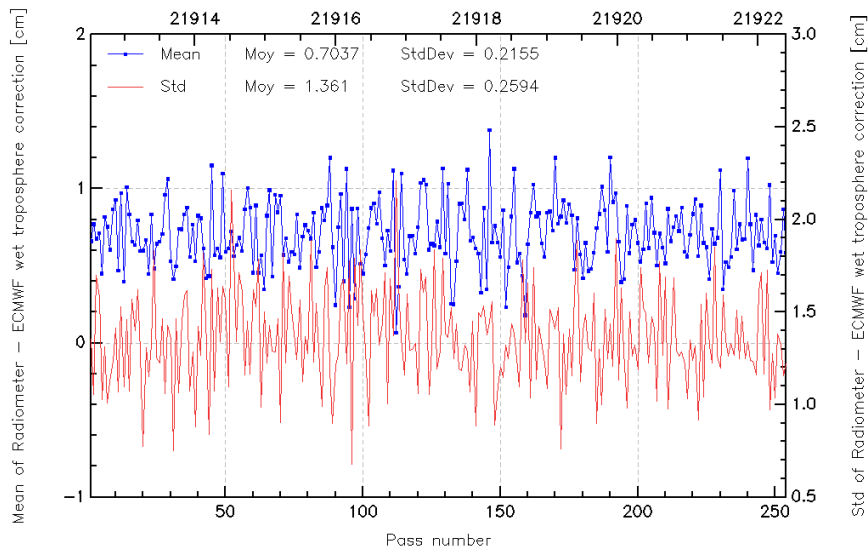
FIG. 11 – Pass monitoring of wet troposphere differences between radiometer and ECMWF model for Jason-2 cycle 055.
