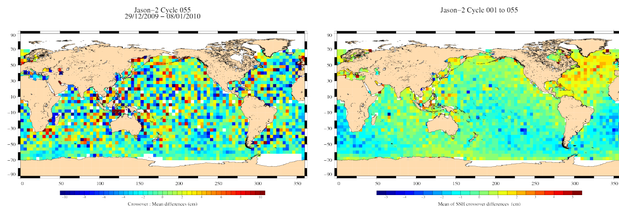
FIG. 13 – Mean SSH at crossovers for cycle 055 (left) and over the whole Jason-2 period (right).
