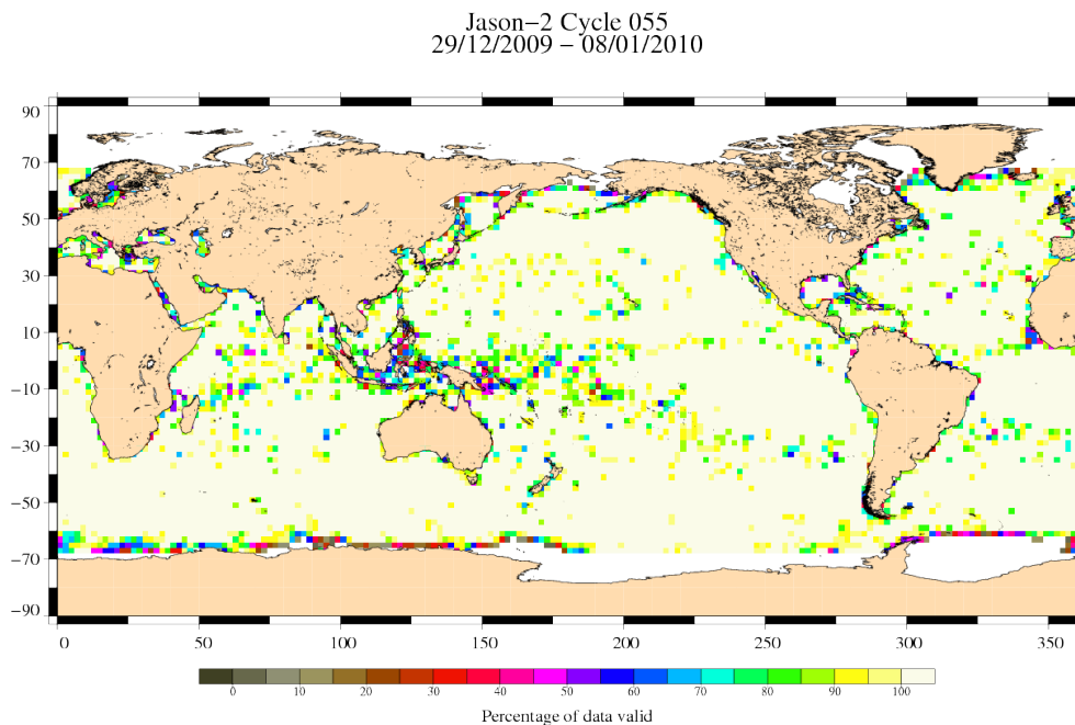
FIG. 3 – Percentage of valid measurements for cycle 055.
