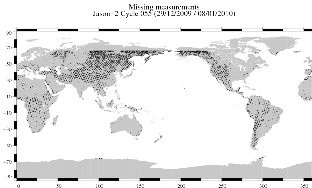
FIG. 1 – Missing measurements for cycle 055.
