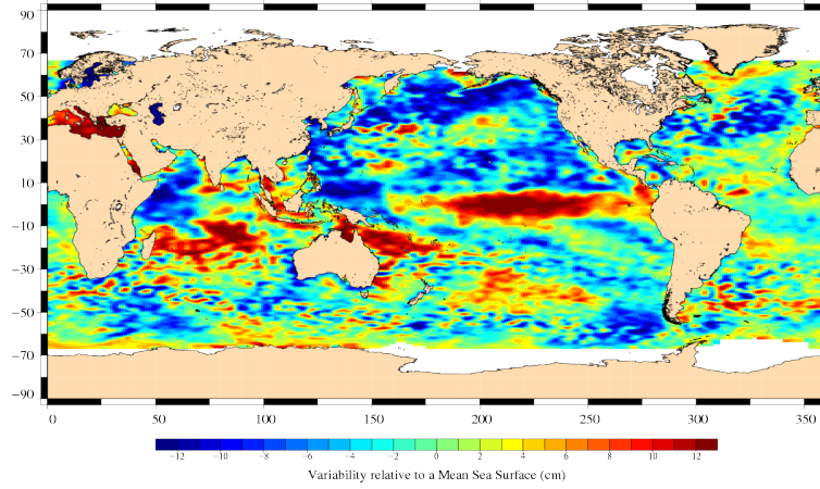
FIG. 18 – Sea level anomaly relative to MSS for cycle 055.
