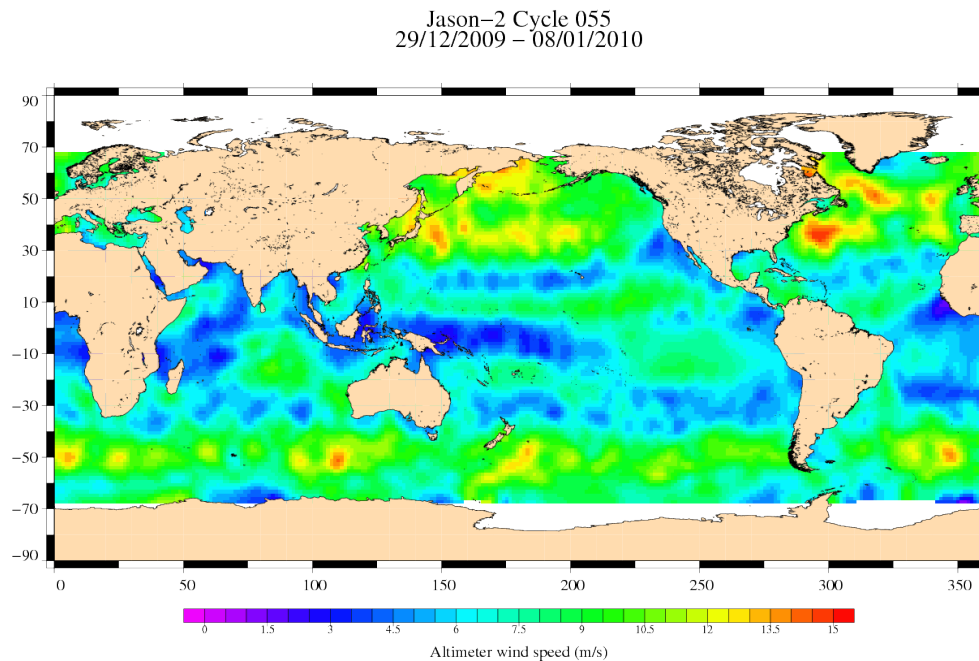
FIG. 9 – Altimeter wind speed for cycle 055.
