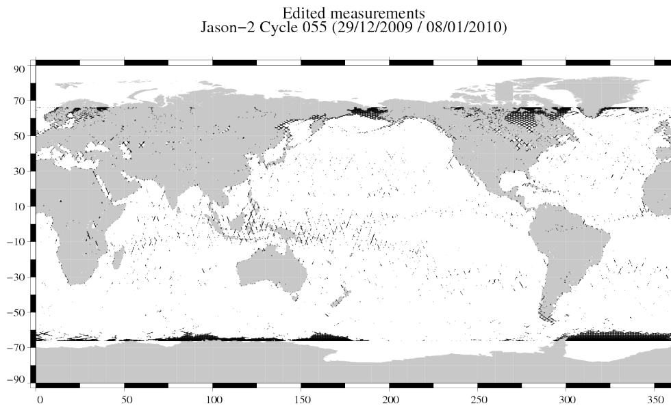
FIG. 2 – Edited measurements for cycle 055.
