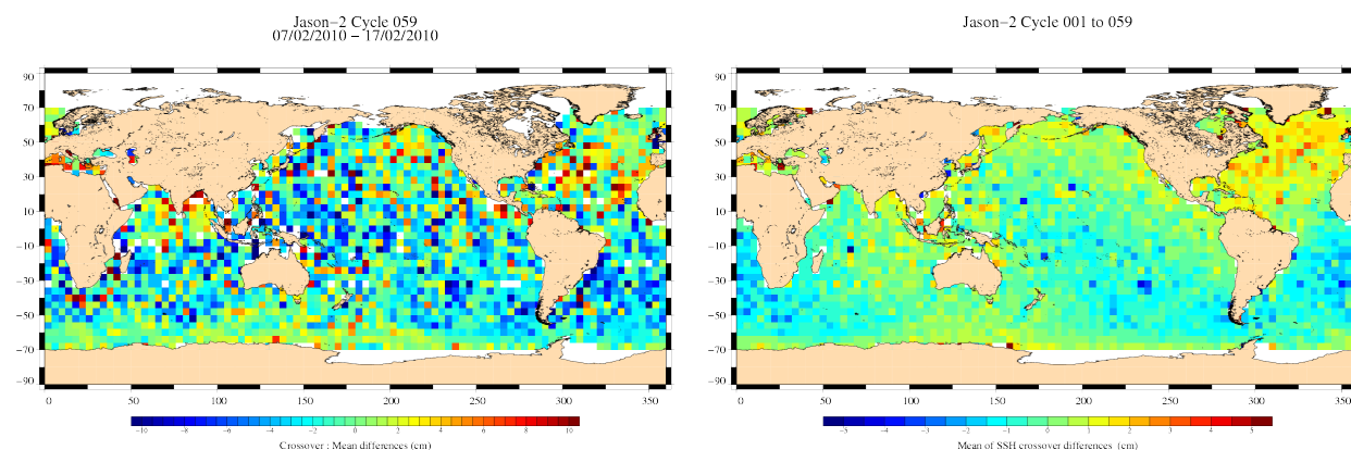
FIG. 13 – Mean SSH at crossovers for cycle 059 (left) and over the whole Jason-2 period (right).
