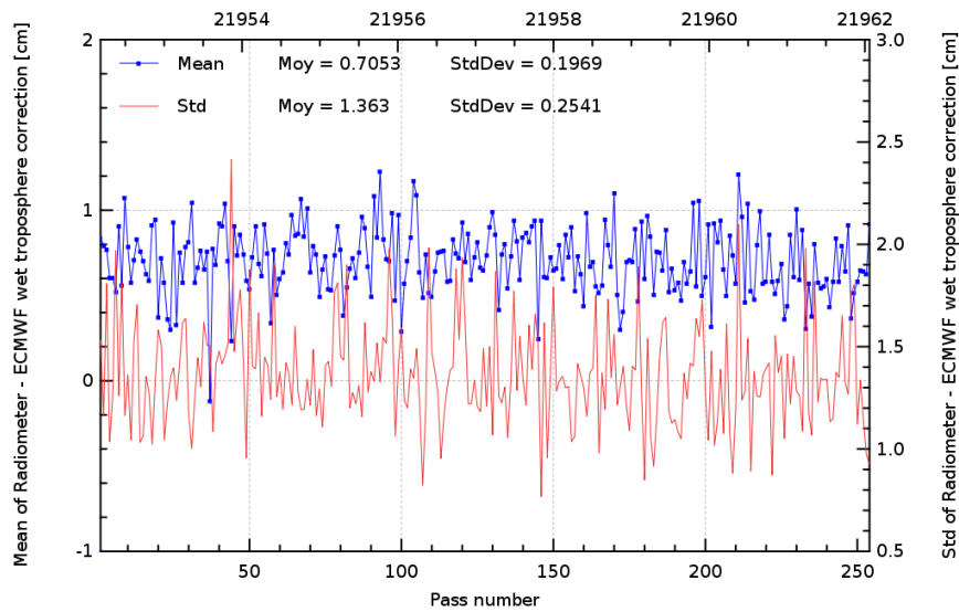
FIG. 11 – Pass monitoring of wet troposphere differences between radiometer and ECMWF model for Jason-2 cycle 059.
