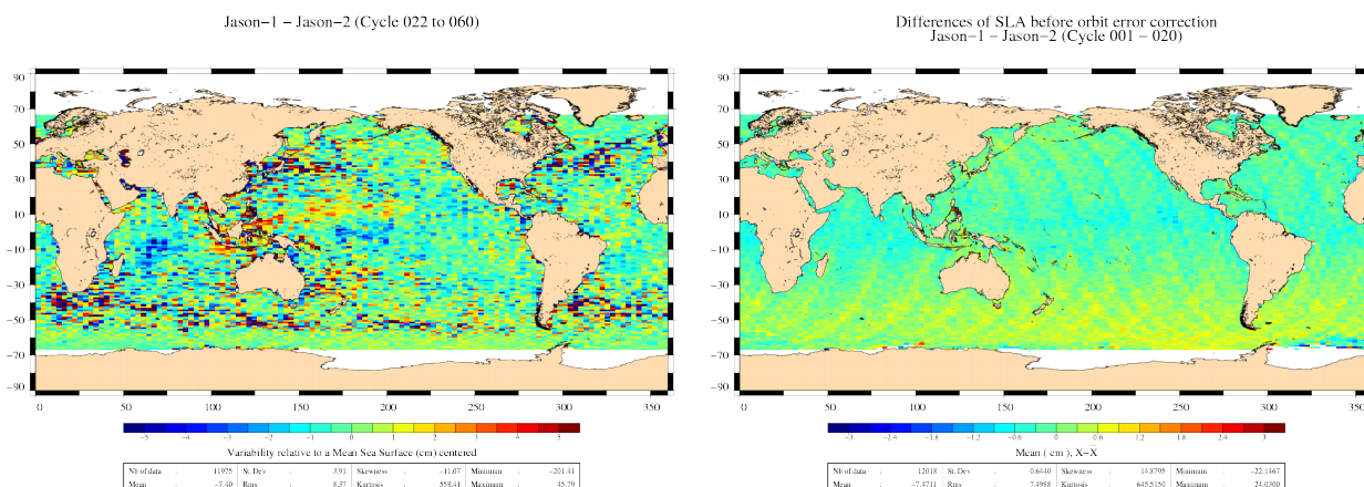
FIG. 20 – Jason-1 – Jason-2 SLA differences averaged over whole Jason-2 period since cycle 022 (left), and for flight formation phase (cycle 001 to 020) (right).
