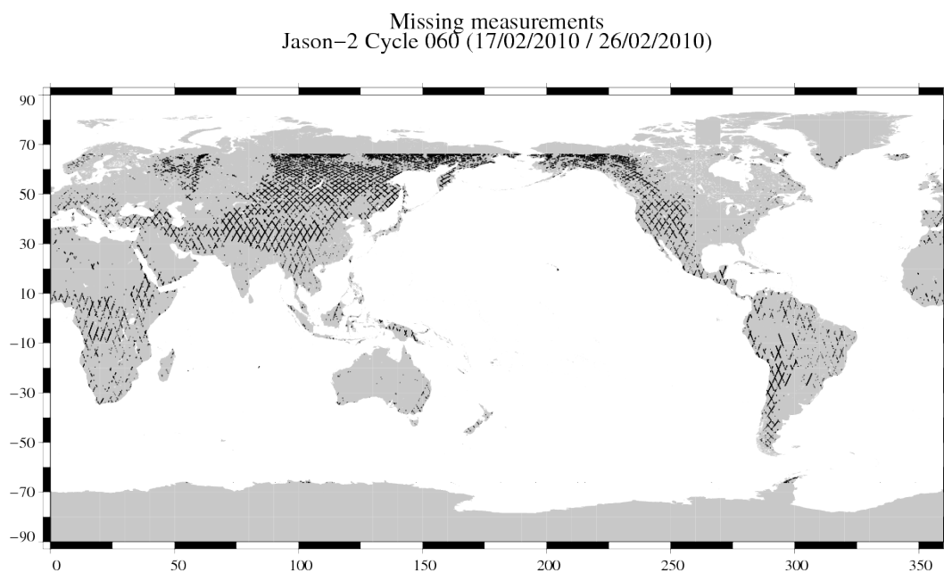
FIG. 1 – Missing measurements for cycle 060.
