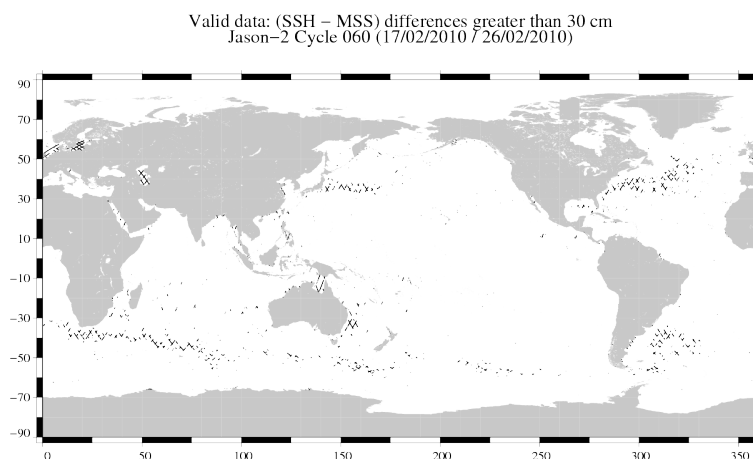
FIG. 19 – Differences higher than a 30 cm threshold for cycle 060.
