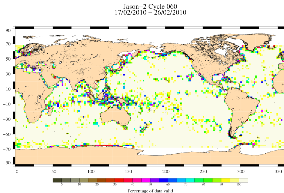
FIG. 3 – Percentage of valid measurements for cycle 060.
