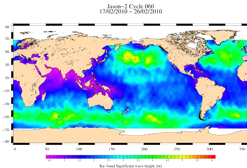
FIG. 5 – Significant wave height for cycle 060.
