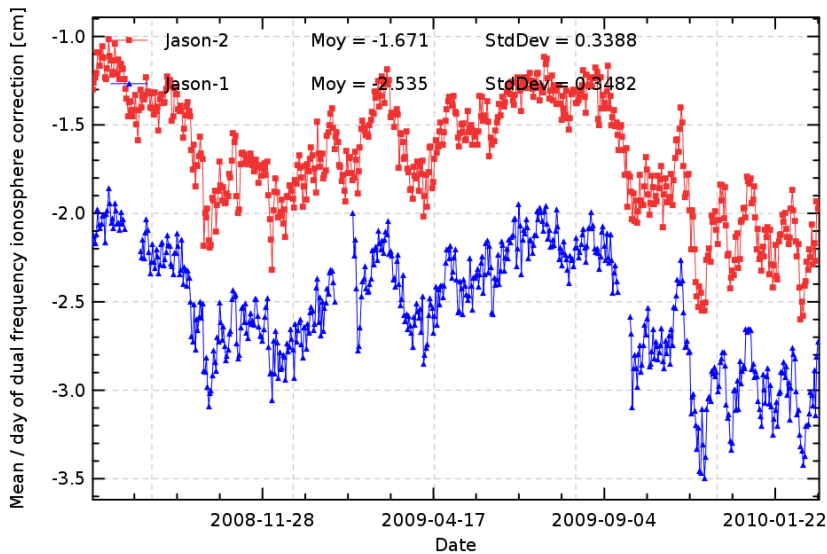
FIG. 8 – Daily monitoring of dual-frequency ionosphere correction for Jason-2 and Jason-1.
