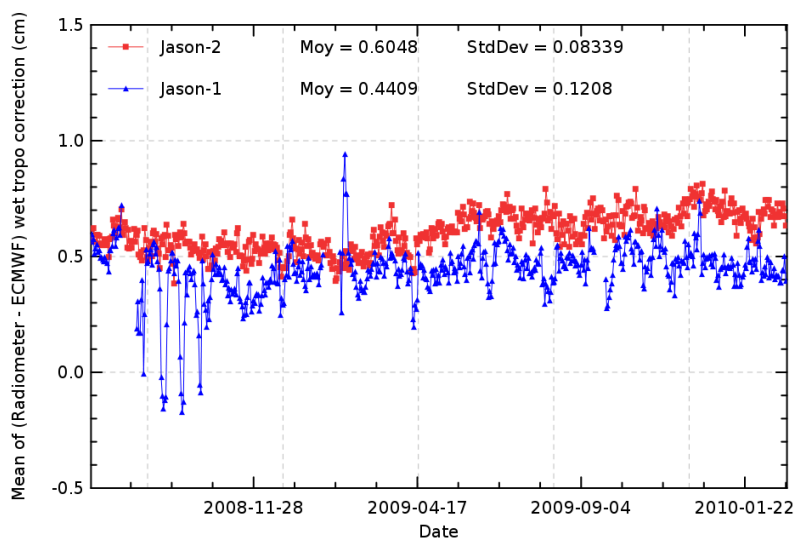
FIG. 12 – Daily monitoring of wet troposphere differences between radiometer and ECMWF model
