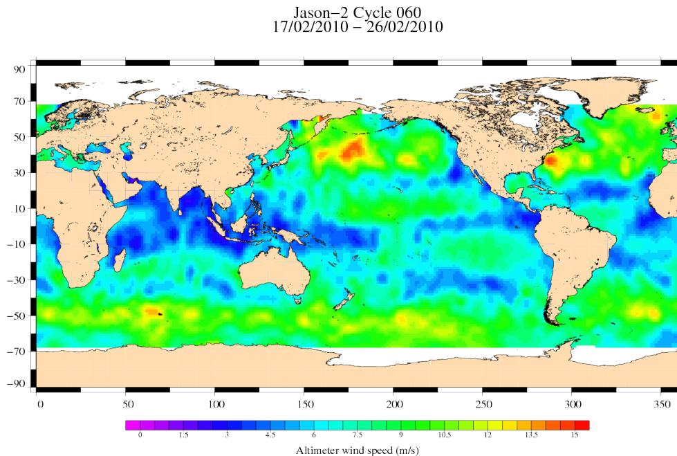
FIG. 9 – Altimeter wind speed for cycle 060.
