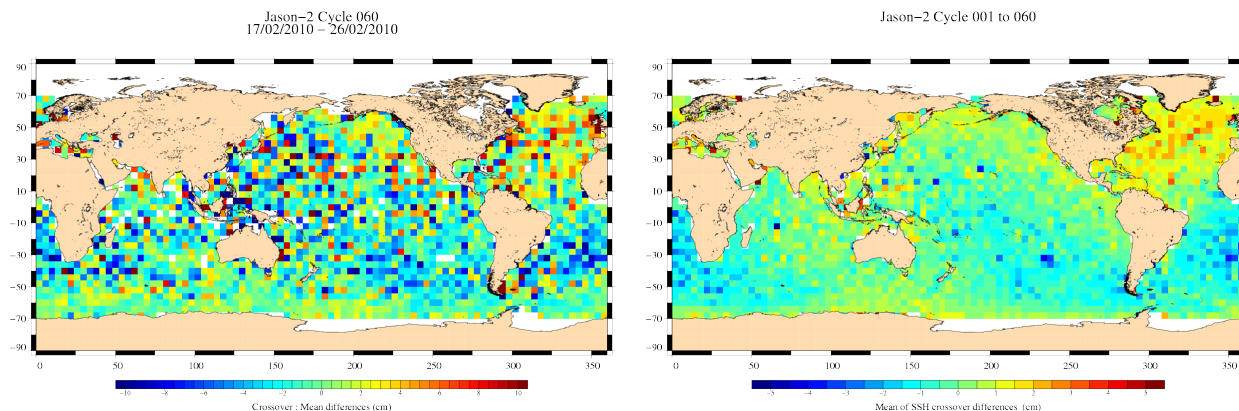
FIG. 13 – Mean SSH at crossovers for cycle 060 (left) and over the whole Jason-2 period (right).
