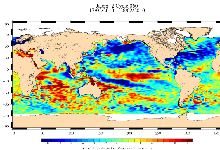
FIG. 18 – Sea level anomaly relative to MSS for cycle 060.
