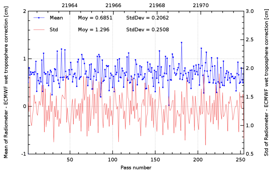
FIG. 11 – Pass monitoring of wet troposphere differences between radiometer and ECMWF model for Jason-2 cycle 060.
