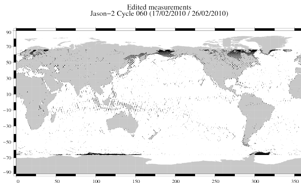
FIG. 2 – Edited measurements for cycle 060.
