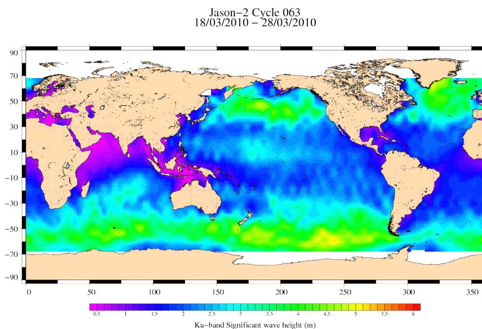
FIG. 5 – Significant wave height for cycle 063.
