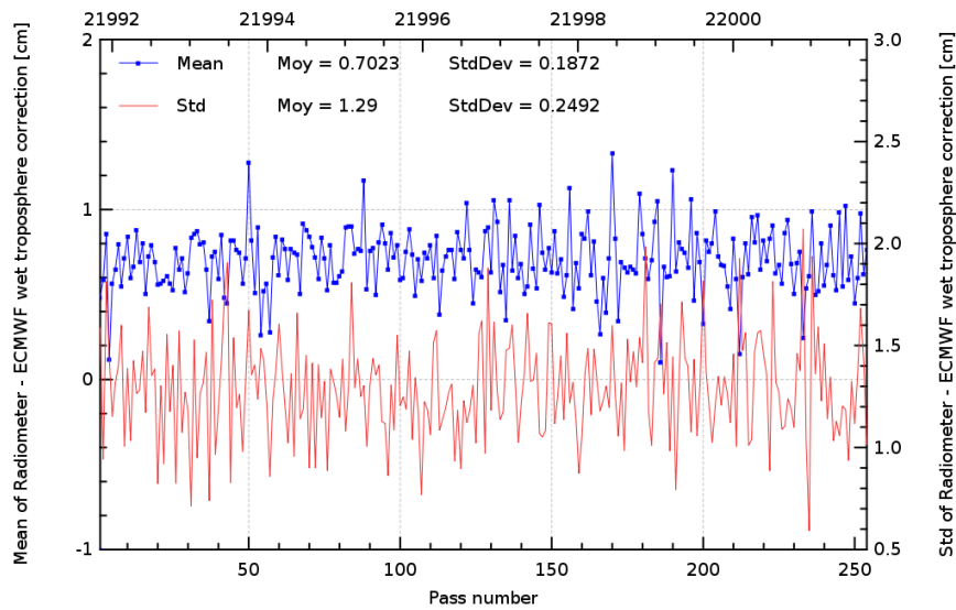
FIG. 11 – Pass monitoring of wet troposphere differences between radiometer and ECMWF model for Jason-2 cycle 063.
