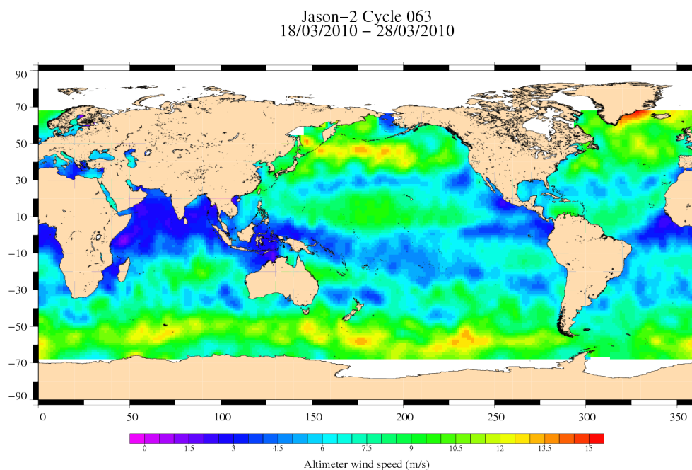
FIG. 9 – Altimeter wind speed for cycle 063.
