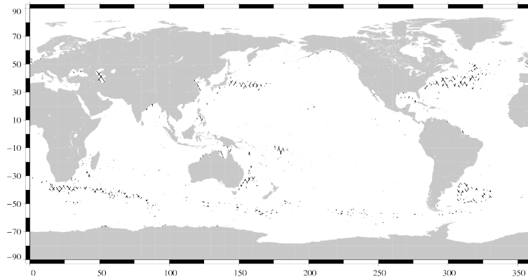
FIG. 19 – Differences higher than a 30 cm threshold for cycle 063.
