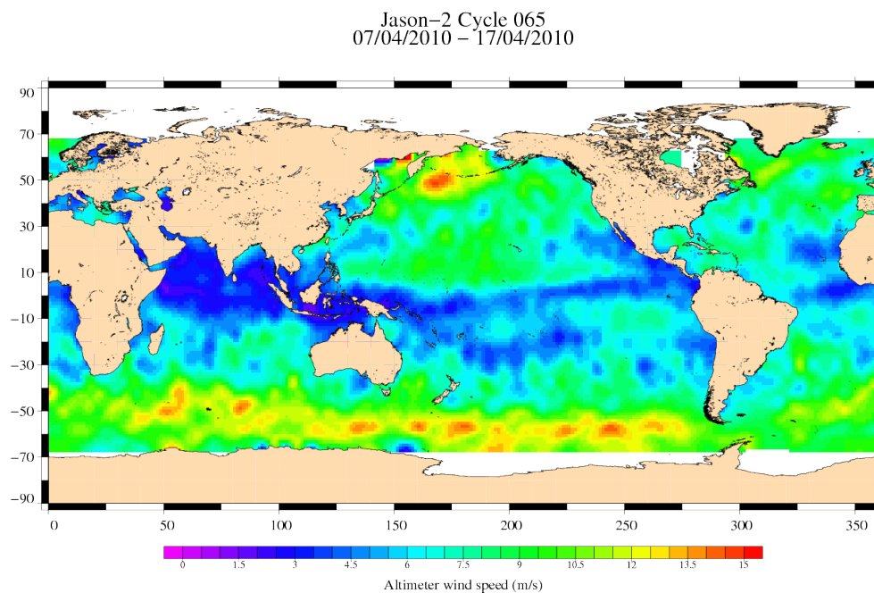
FIG. 9 – Altimeter wind speed for cycle 065.
