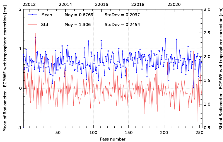
FIG. 11 – Pass monitoring of wet troposphere differences between radiometer and ECMWF model for Jason-2 cycle 065.
