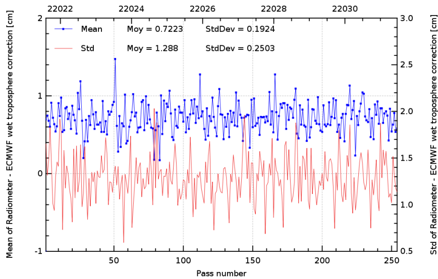
FIG. 11 – Pass monitoring of wet troposphere differences between radiometer and ECMWF model for Jason-2 cycle 066.
