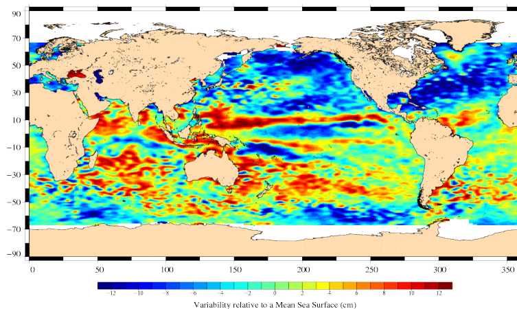
Jason-2 Cycle 066 17/04/2010 – 27/04/2010
