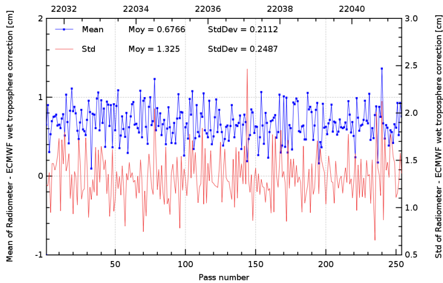
FIG. 11 – Pass monitoring of wet troposphere differences between radiometer and ECMWF model for Jason-2 cycle 067.
