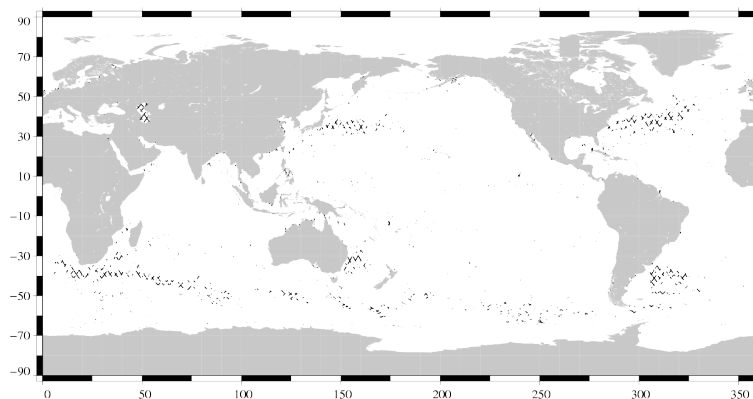
FIG. 19 – Differences higher than a 30 cm threshold for cycle 067.
