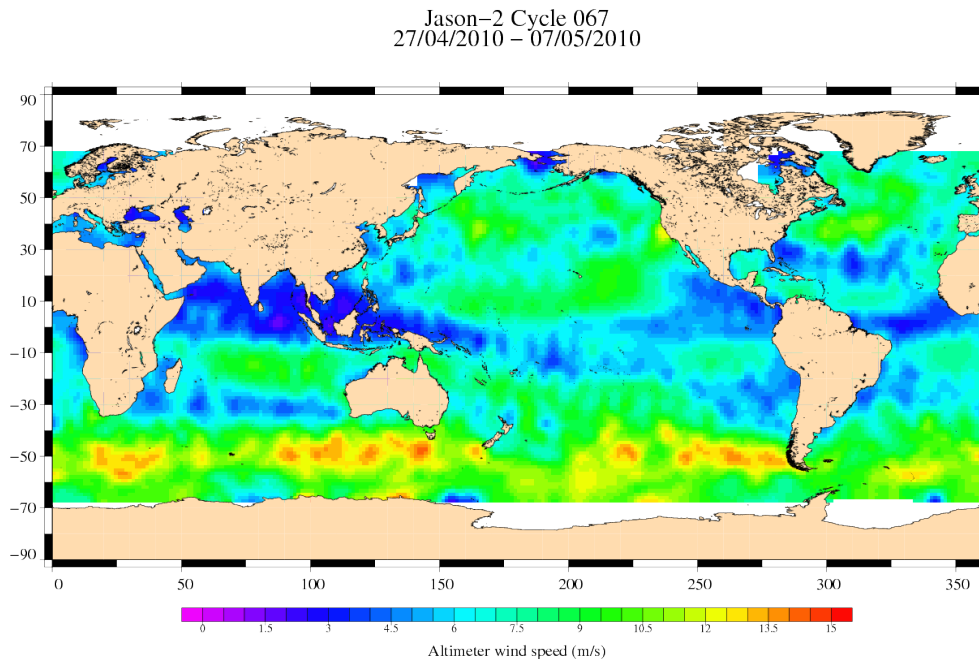
FIG. 9 – Altimeter wind speed for cycle 067.
