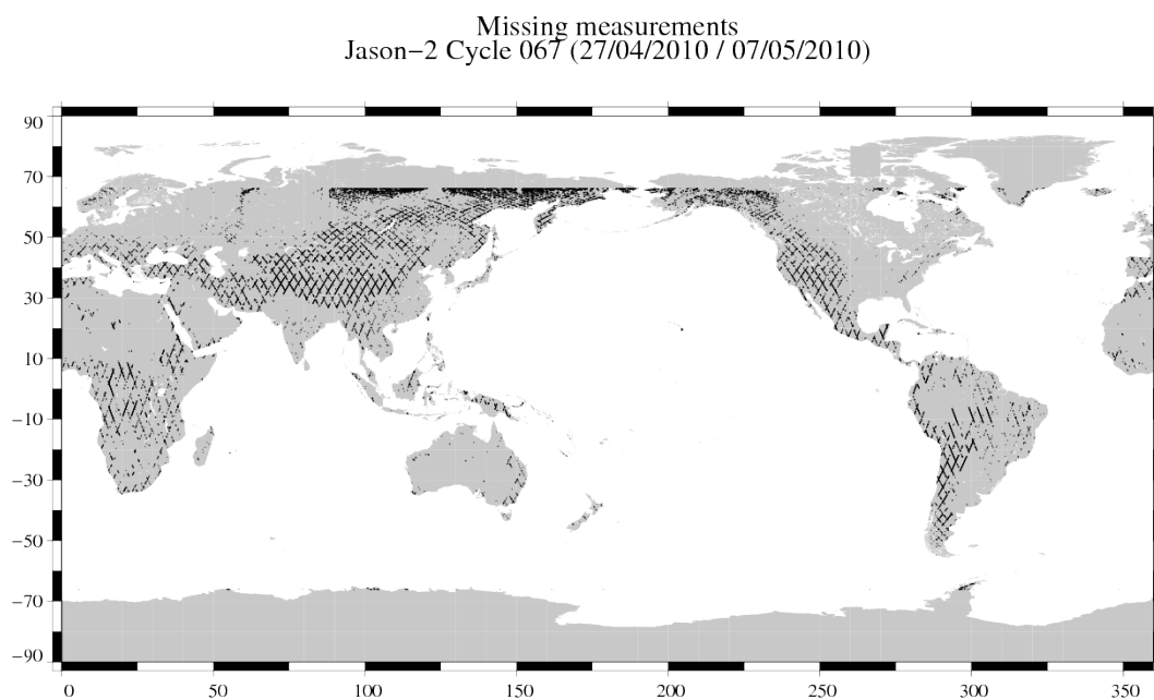
FIG. 1 – Missing measurements for cycle 067.
