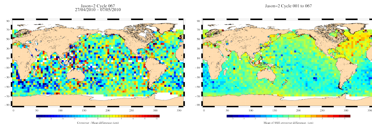
FIG. 13 – Mean SSH at crossovers for cycle 067 (left) and over the whole Jason-2 period (right).
