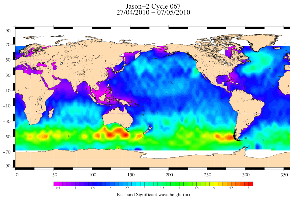
FIG. 5 – Significant wave height for cycle 067.
