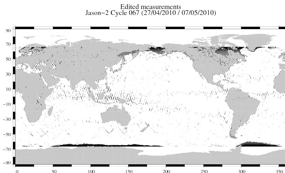
FIG. 2 – Edited measurements for cycle 067.
