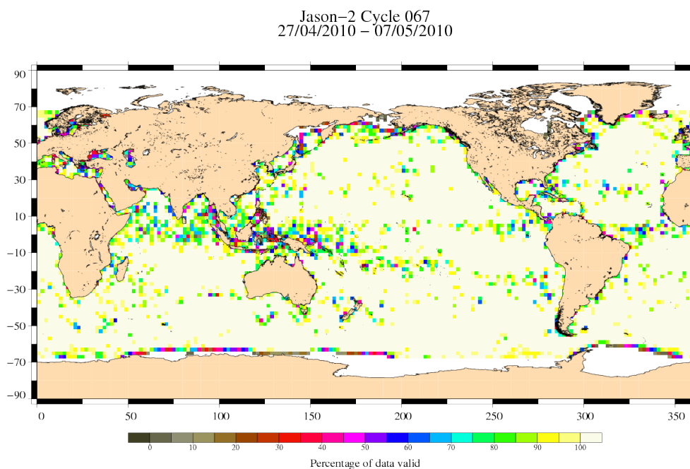
FIG. 3 – Percentage of valid measurements for cycle 067.
