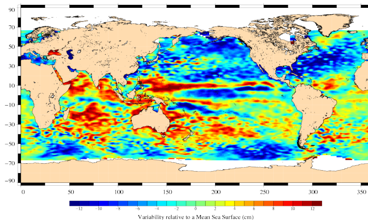
FIG. 18 – Sea level anomaly relative to MSS for cycle 067.
